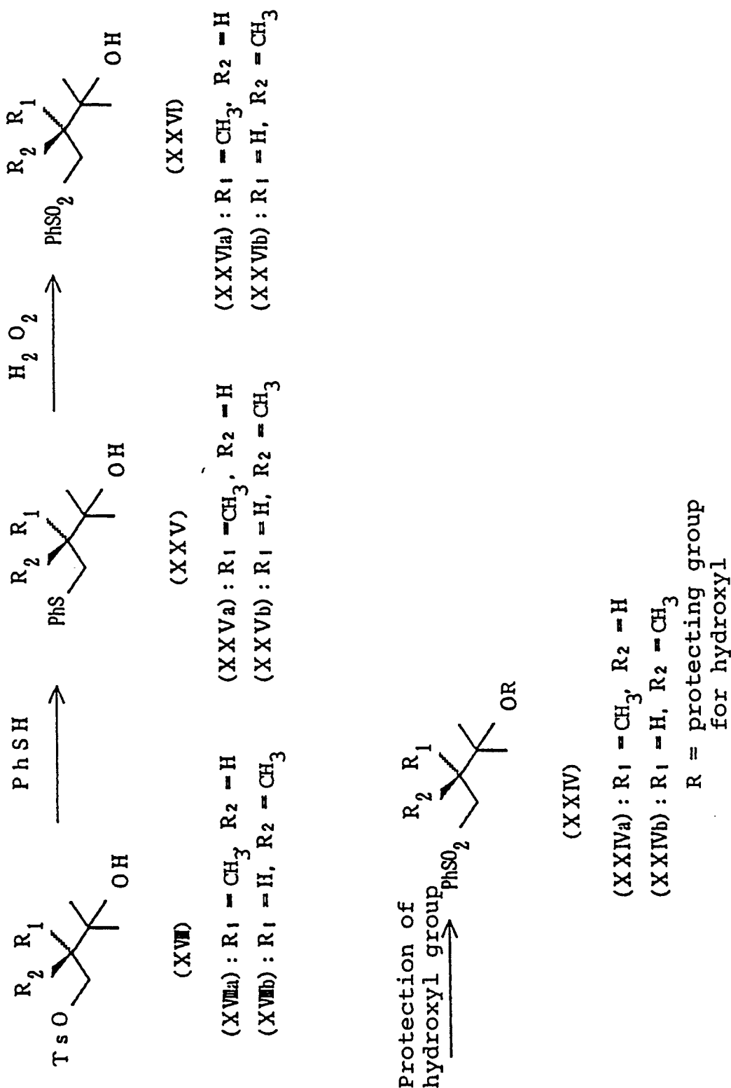
SCHEME V
