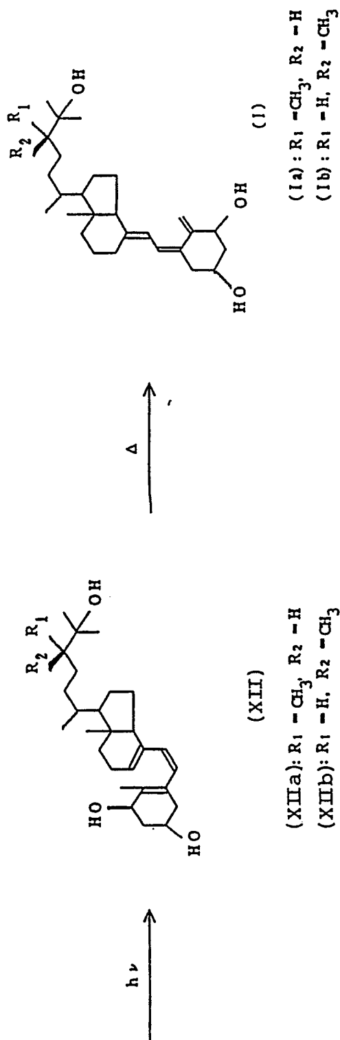
SCHEME I (continued)
