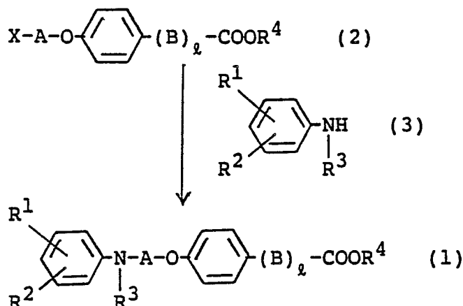
[Reaction Scheme-1]
