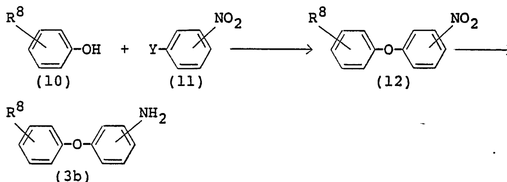
[Reaction Scheme-9]
