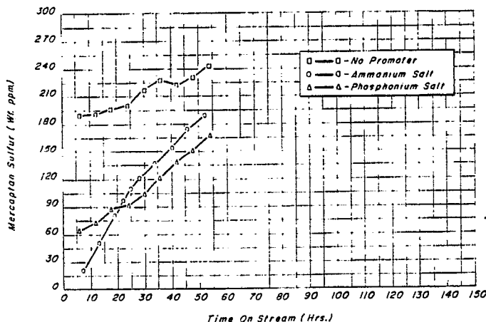
Effect Of Phosphonium Salt On The Oxidation Of Mercaptans.
