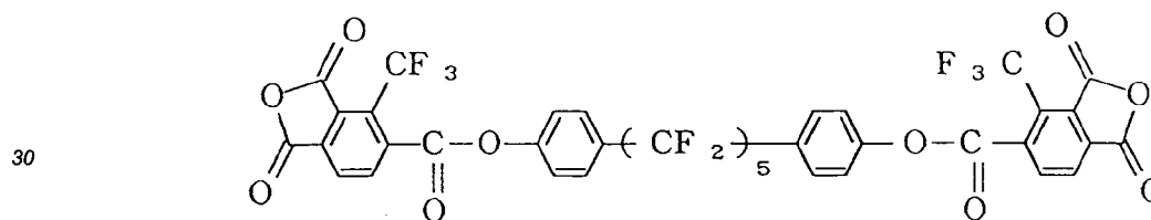
25 VI-(12): 1,5-bis[4-(2-trifluoromethyl-3,5-dicarboxybenzoyloxyphenyl)]decafluoropentane anhydride
