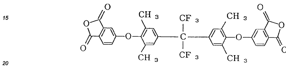
25 VII-(10): 2,2-bis[4-(3,4-dicarboxyphenoxy)phenyl]octafluorobutane anhydride
