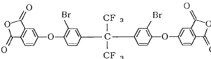
VII-(7): 2,2-bis[4-(3,4-dicarboxyphenoxy)-3-bromophenyl]hexafluoropropane anhydride
