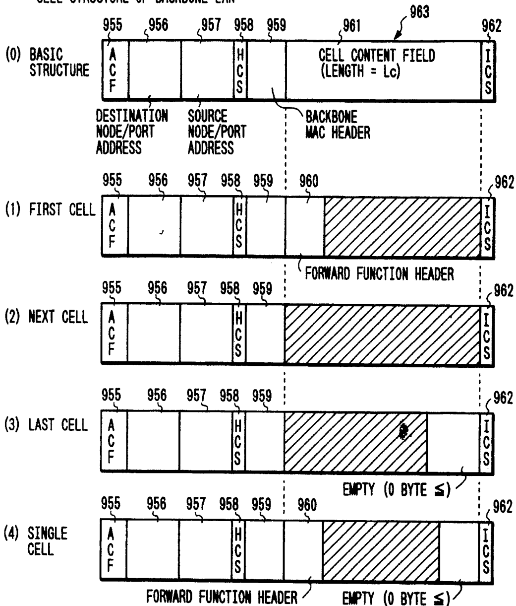
CELL STRUCTURE OF BACKBONE LAN FIG. 2B
