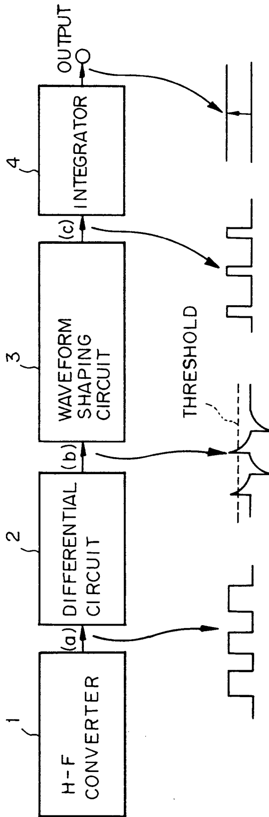
Fig. 15 PRIOR ART
