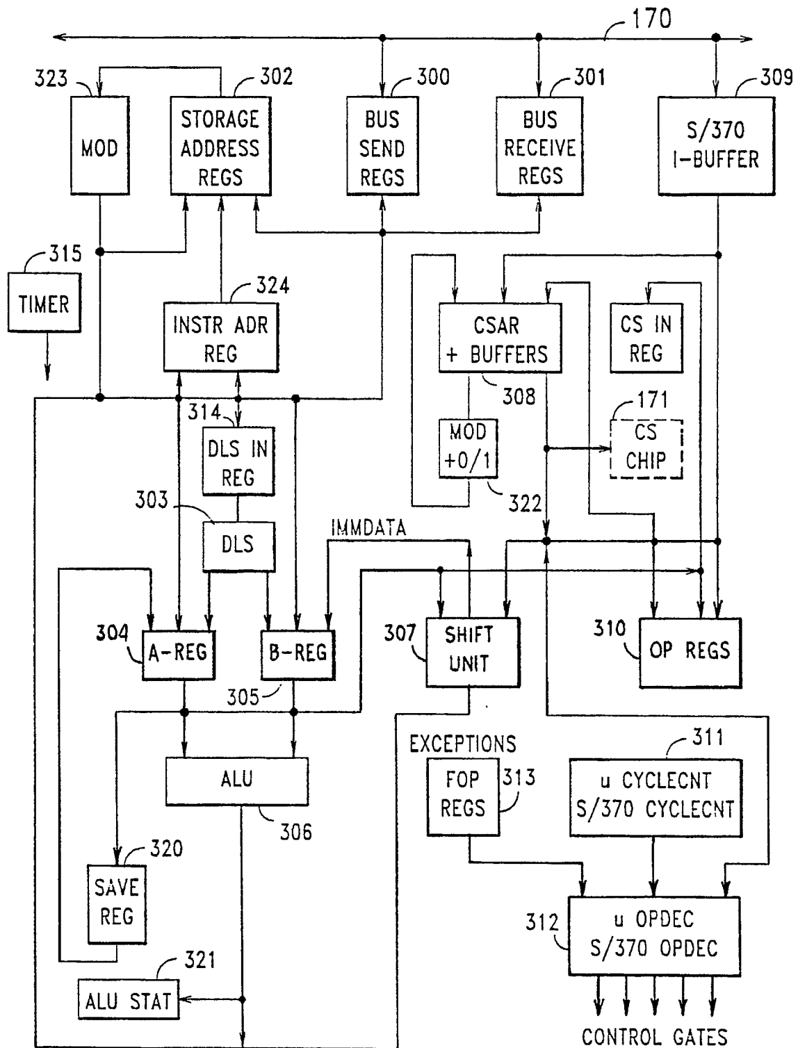
FIG. 27 - S/370 PROCESSOR 85
