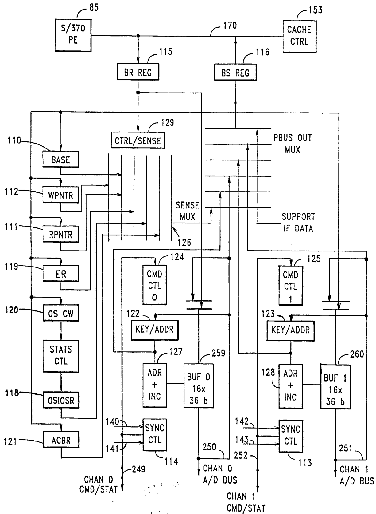
FIG. 13 - BUS ADAPTER 154
