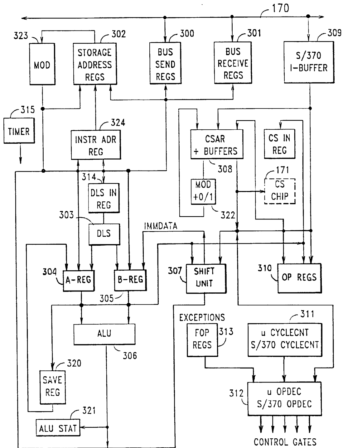
FIG. 27 — S/370 PROCESSOR 85
