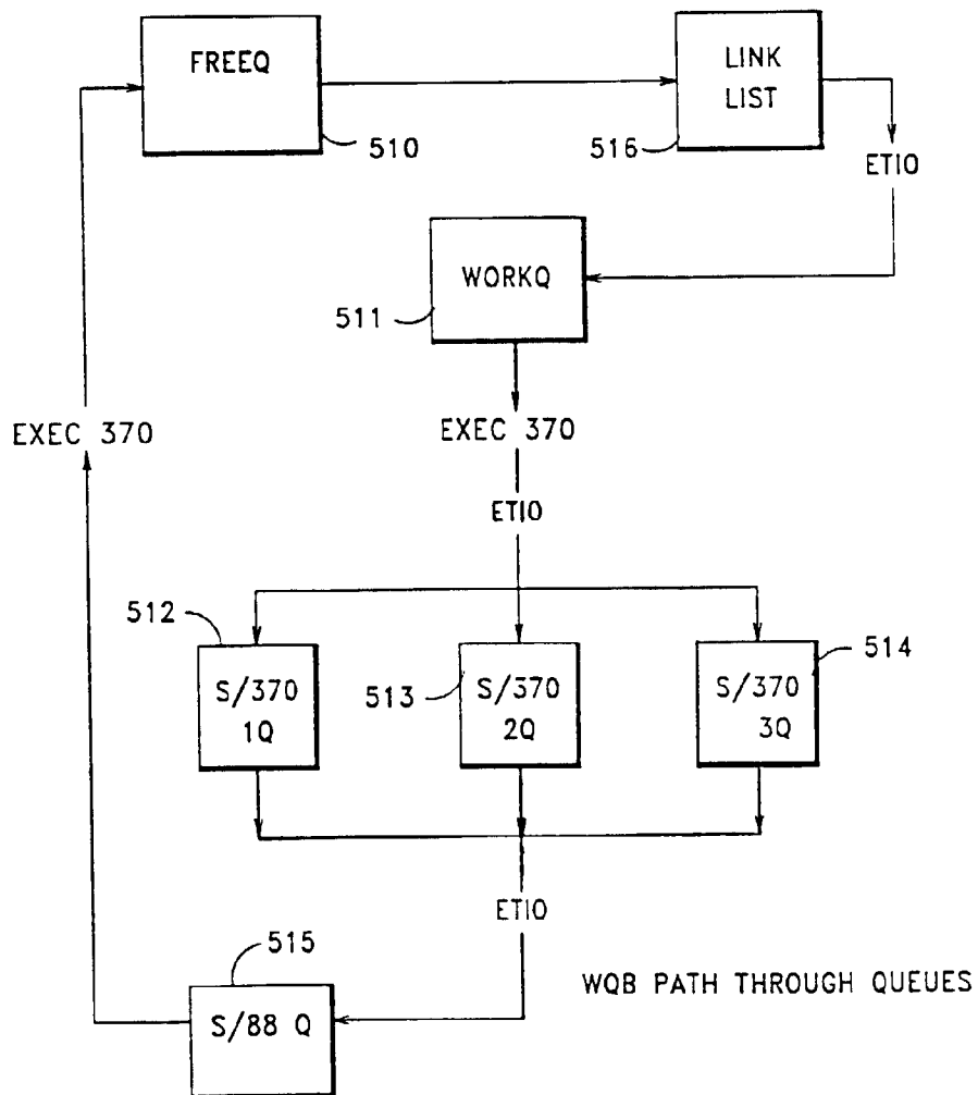
FIG. 41E - WQB PATH THROUGH QUEUES
