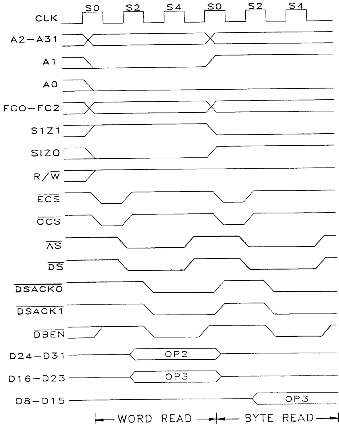
BYTE AND WORD READ CYCLE TIMING (32-BIT DATA PORT) FIG. 22
