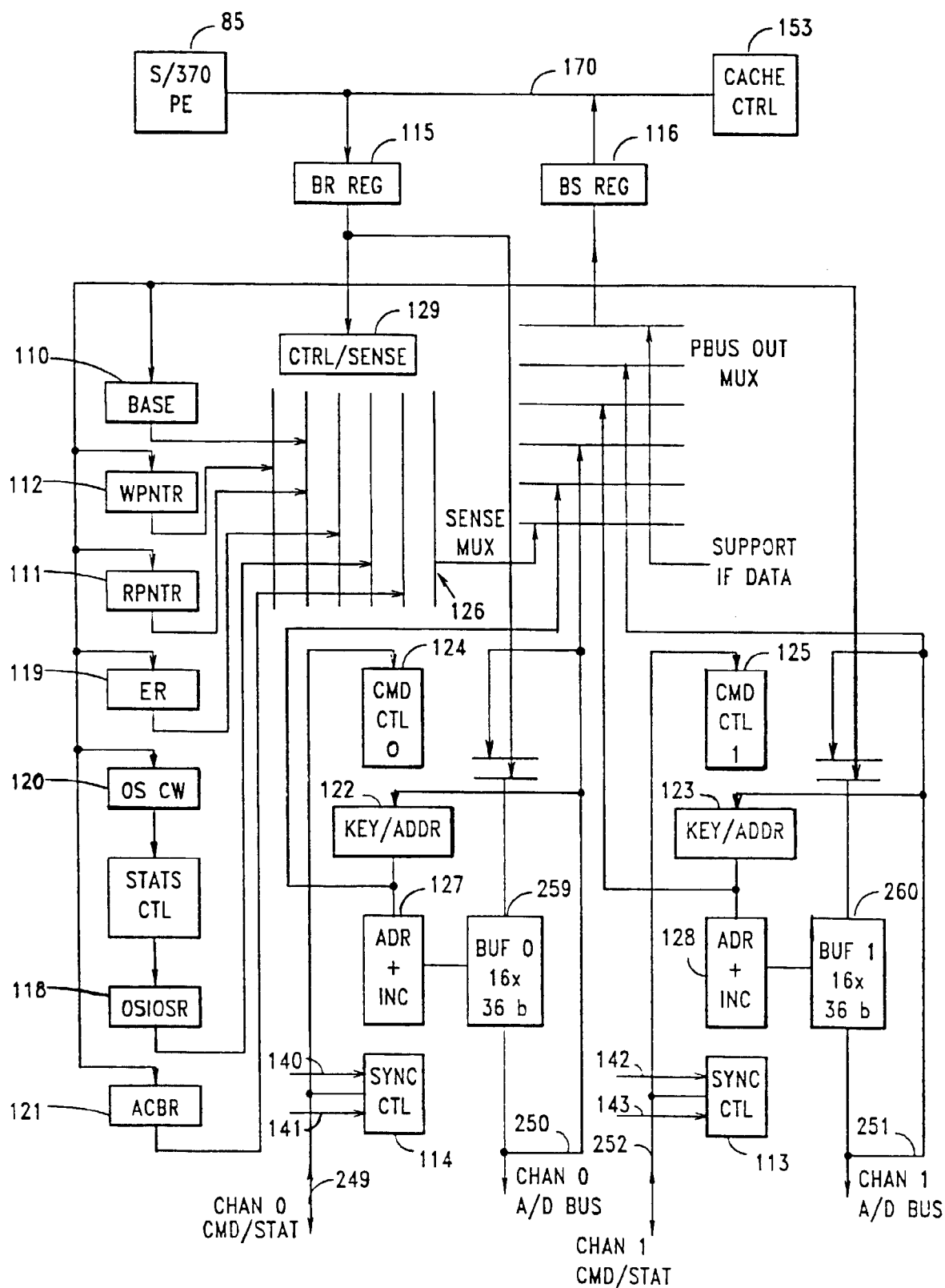
FIG. 13 - BUS ADAPTER 154
