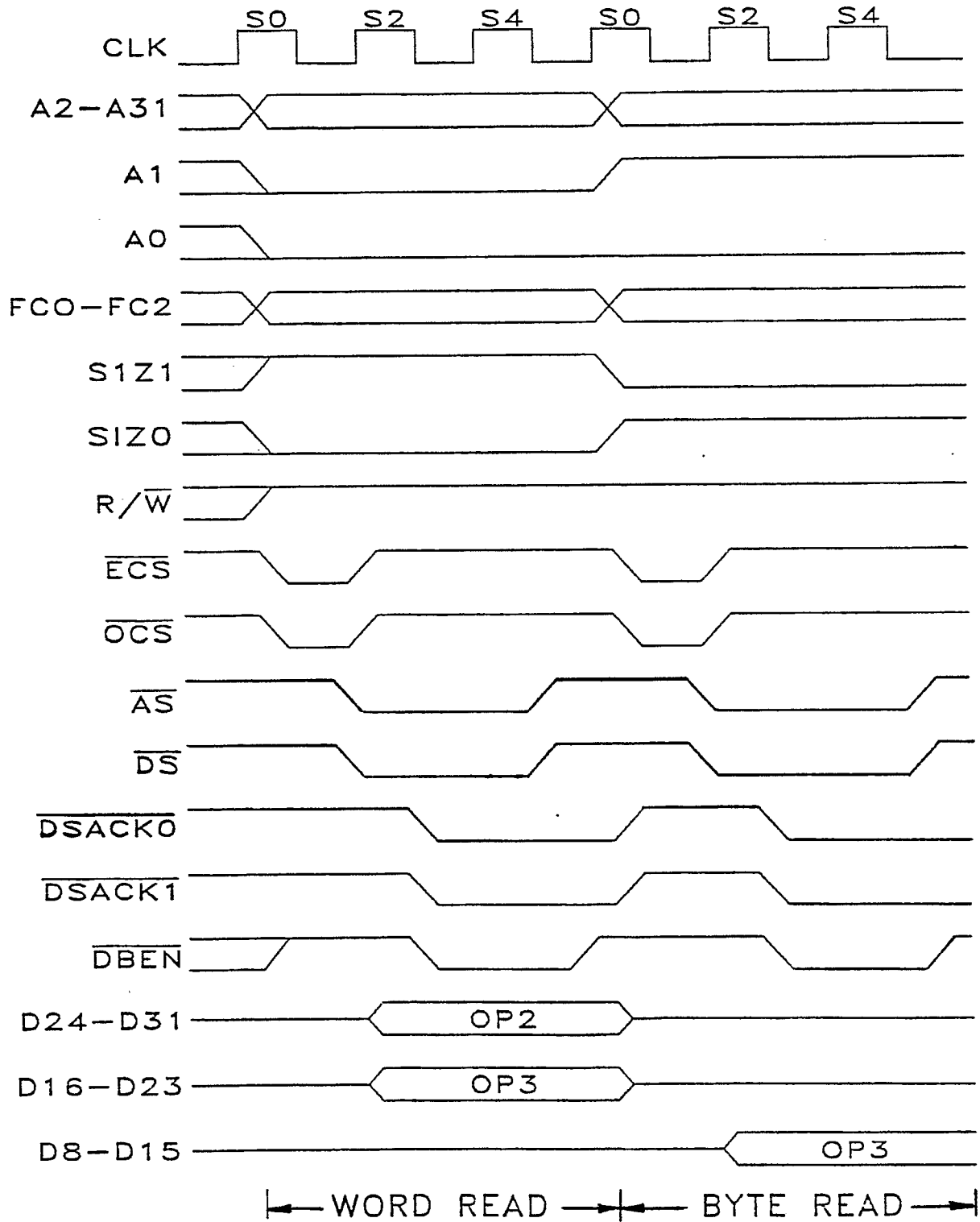
BYTE AND WORD READ CYCLE TIMING (32-BIT DATA PORT)
