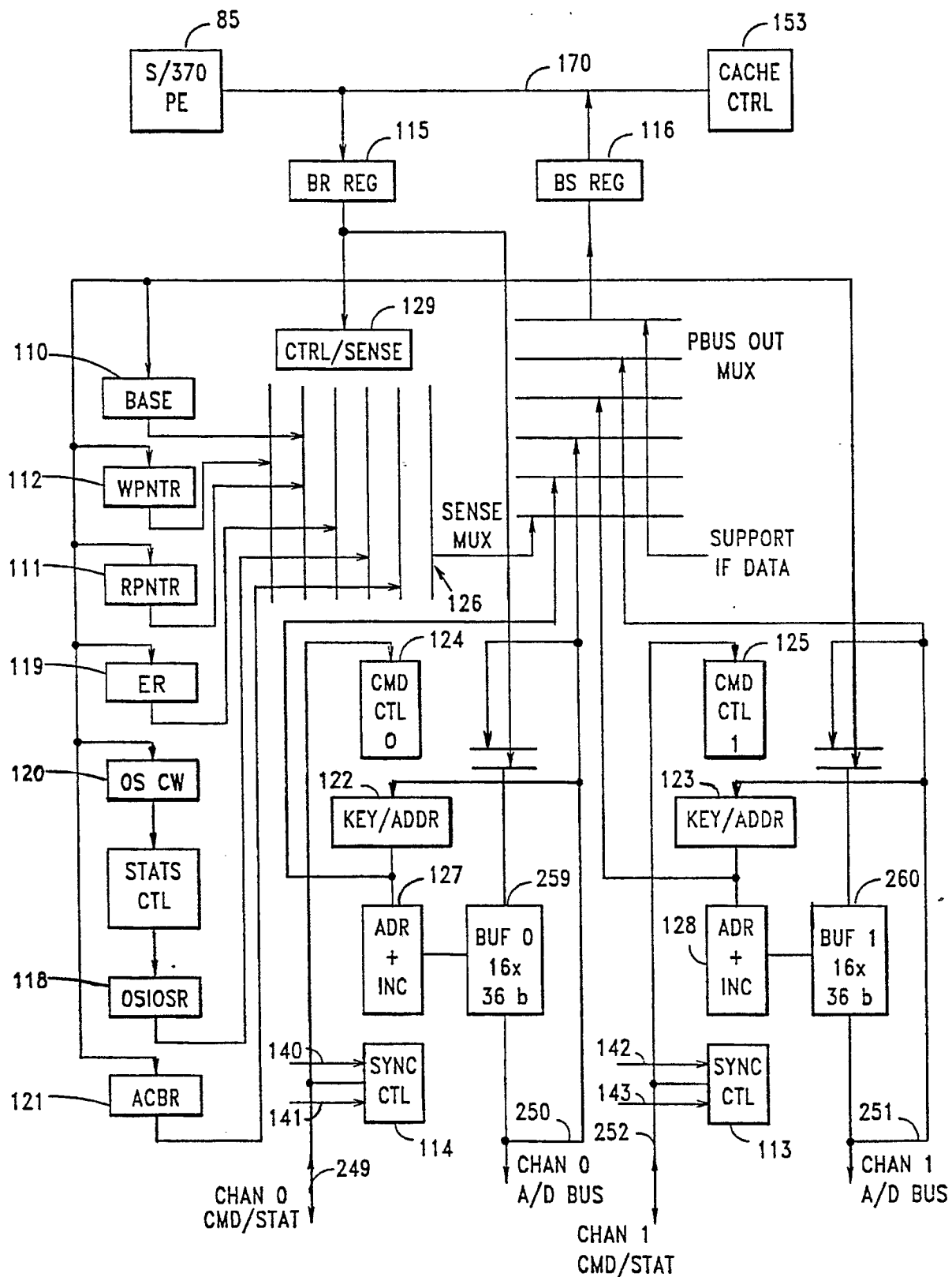
FIG. 13 - BUS ADAPTER 154
