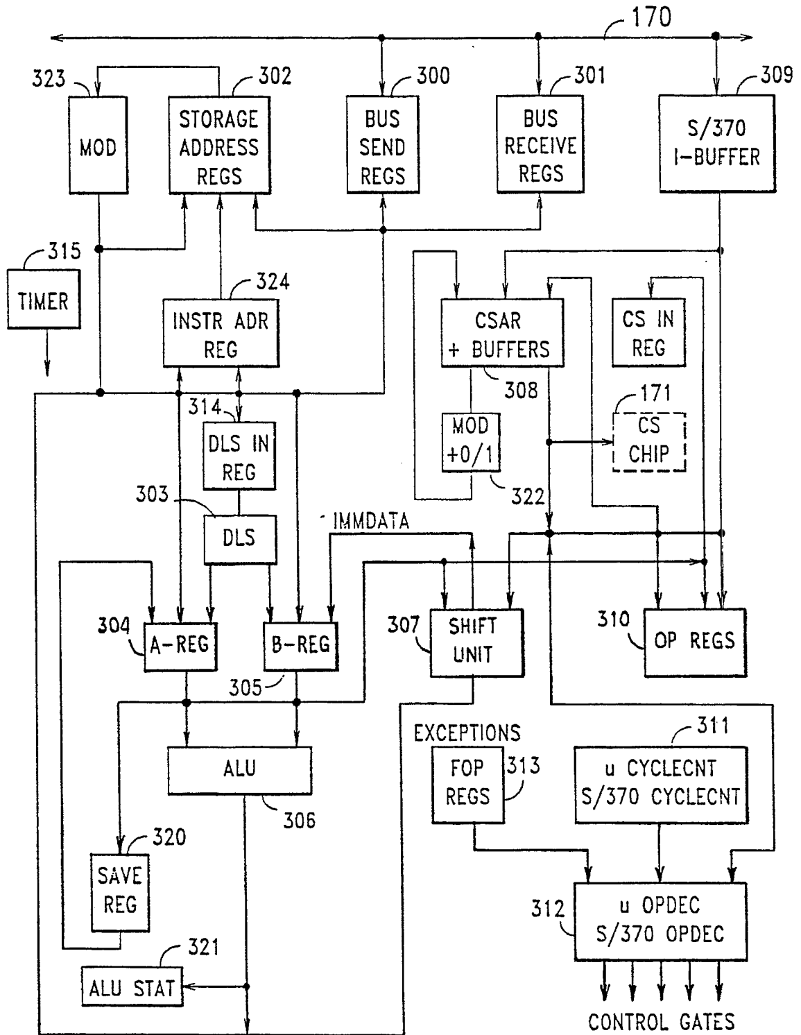
FIG. 27 - S/370 PROCESSOR 85
