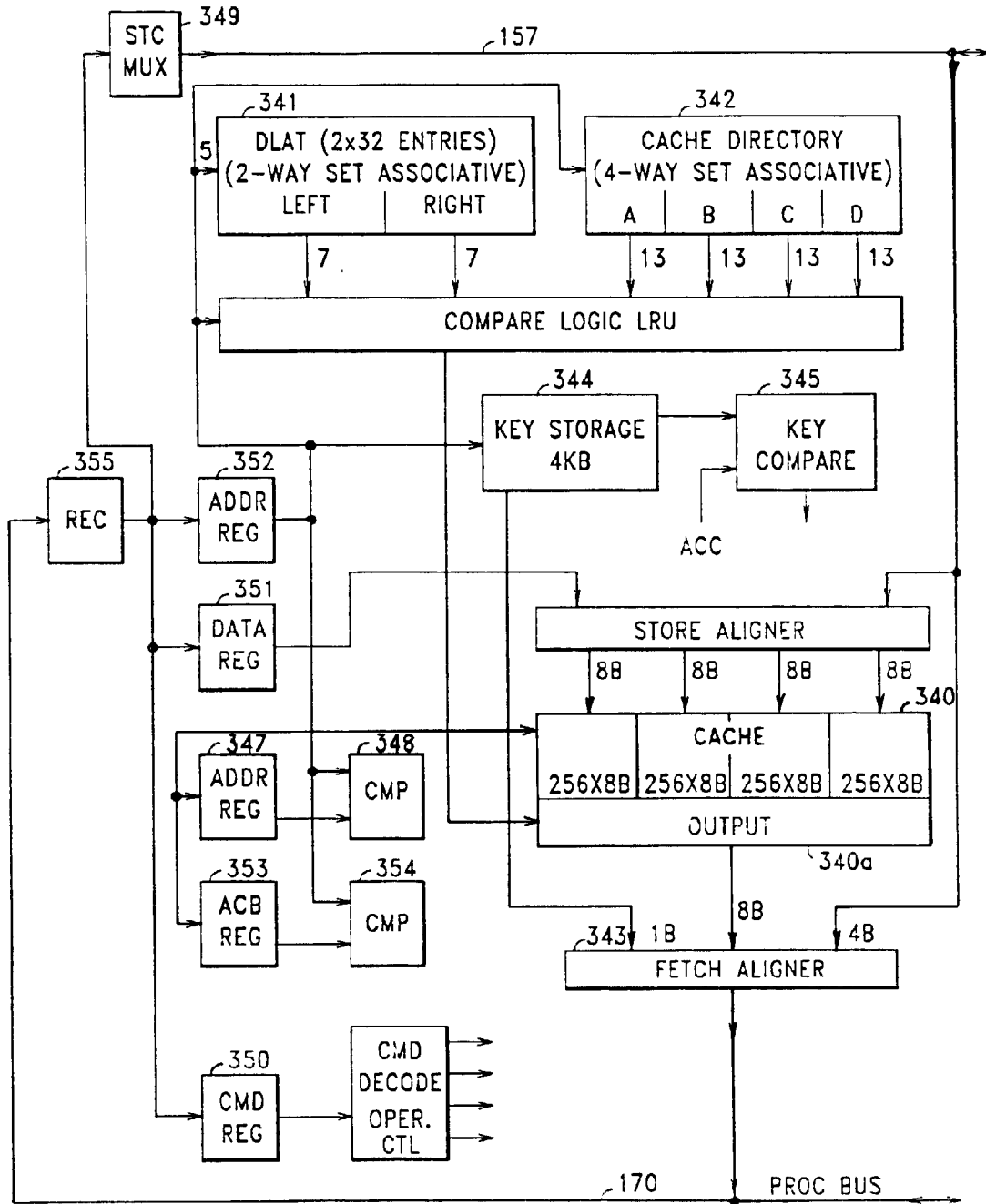
FIG. 31 — CACHE CONTROLLER 153
