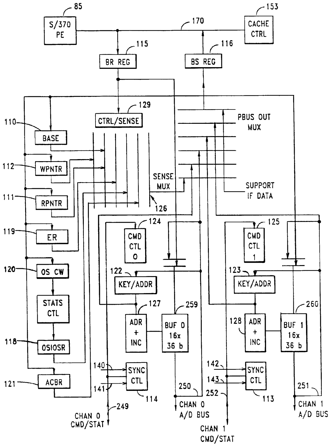
FIG. 13 - BUS ADAPTER 154
