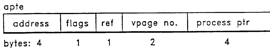
FIG. 48E — Active Page Table Entry
