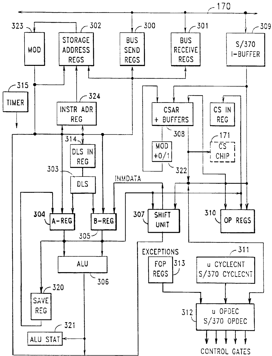
FIG. 27 — S/370 PROCESSOR 85
