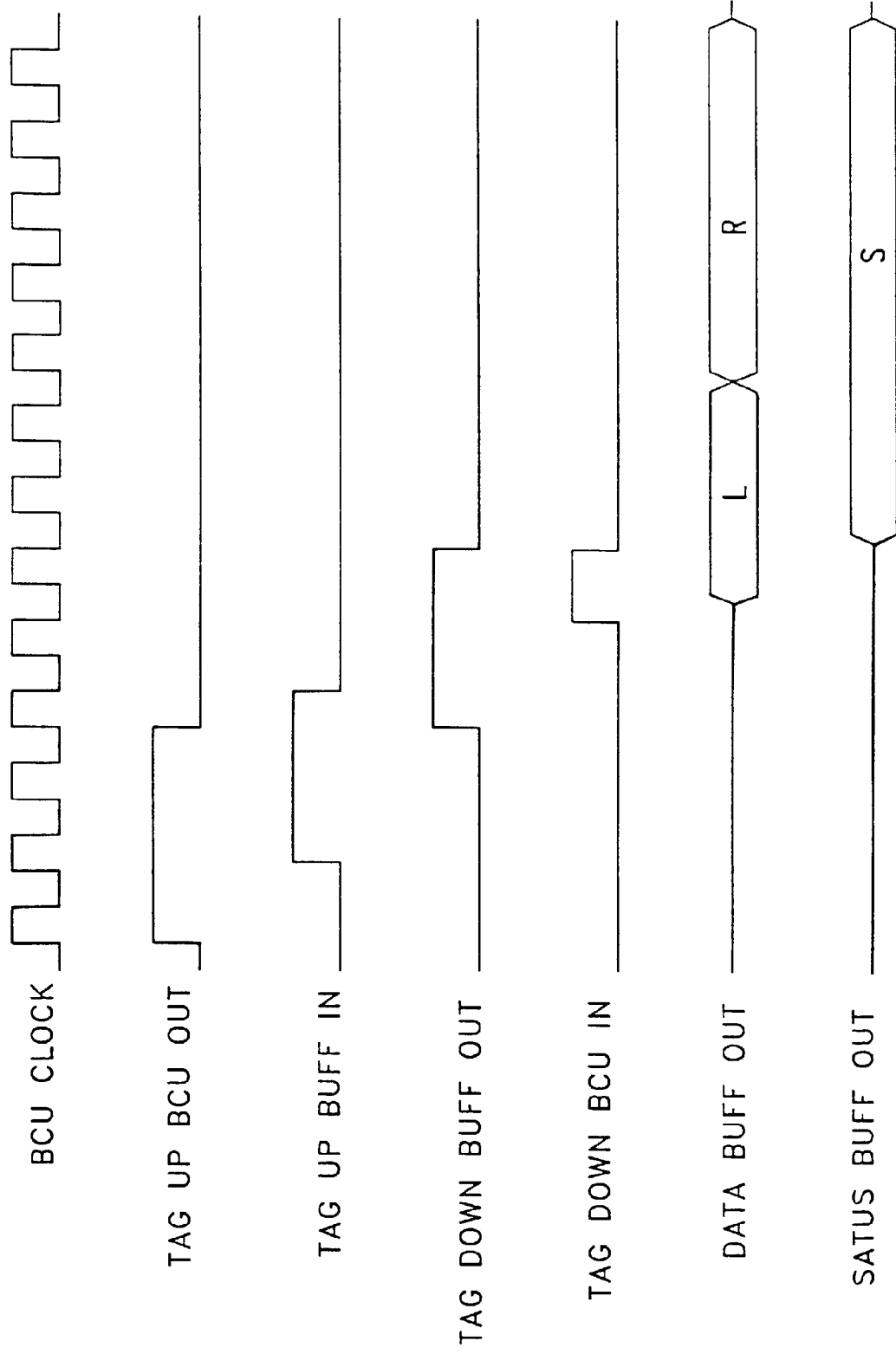
FIG. 15C — FETCH (DATA DELAYED)
