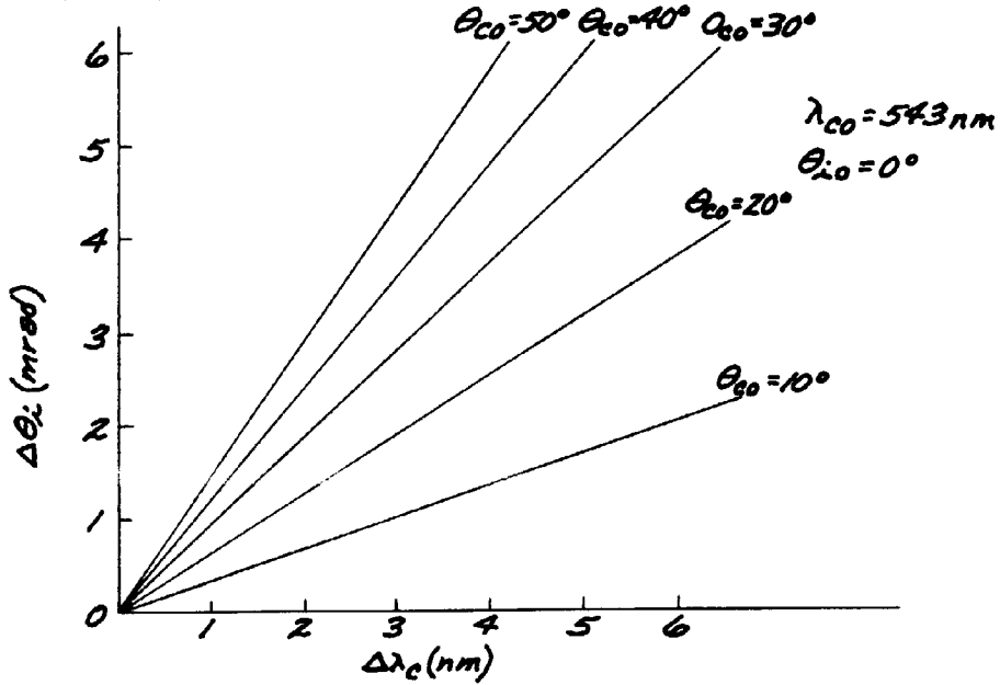
(a) IMAGE BLUR \Delta\theta_i AT HOLOGRAM VS. SPECTRAL BANDWIDTH \Delta\lambda_c (APPLIES TO BOTH REFLECTION AND TRANSMISSION HOLOGRAMS)
