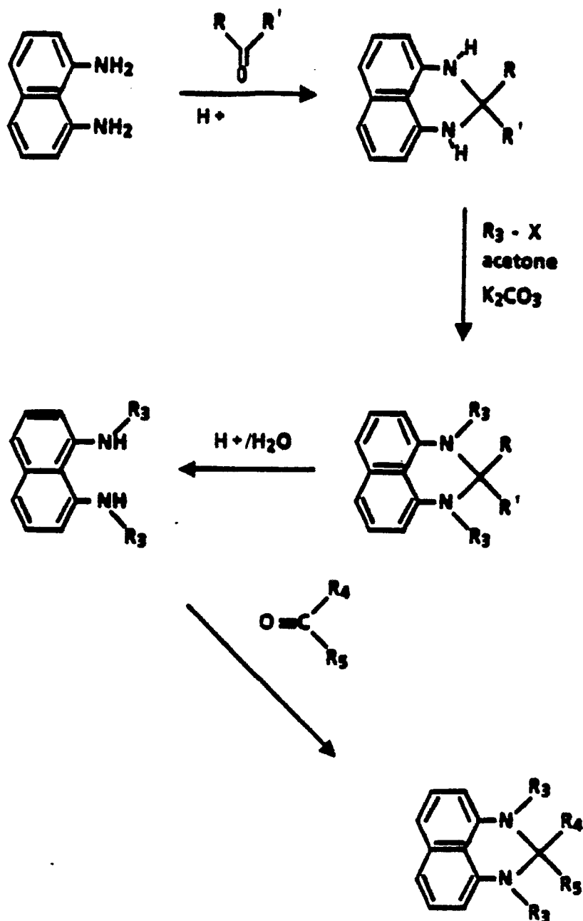
Figure 6 - New route to N,N'-dialkyl-1,8-naphthalene diamines, with subsequent condensation to N,N'-dialkyl-2,3-dihydro-2,2-dialkyl or 2-alkyl perimidine.
