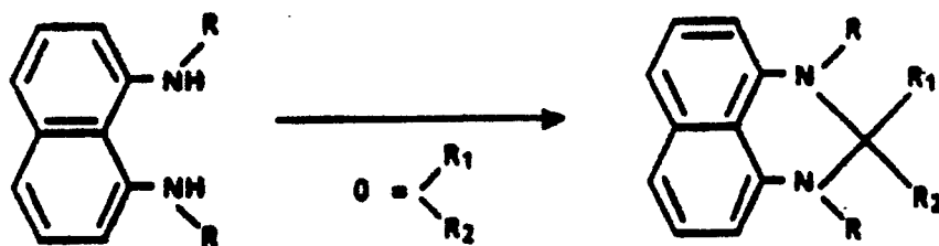
Figure 2 - Condensation of N,N'-dialkyl-1,8-naphthalene diamine with aldehyde or ketone to form 2,3-dihydro-1,3-dialkyl perimidines
