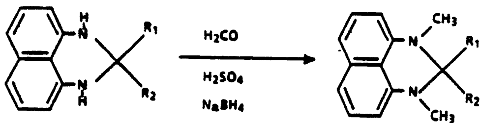
Figure 4 - New reductive methylation of 2,3-dihydro-2,2-dialkyl perimidine.
