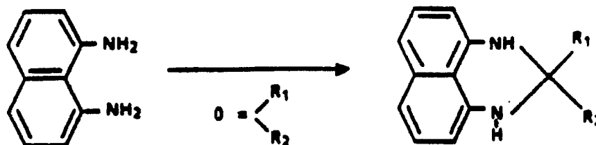
Figure 1 - Condensation of 1,8-naphthalene diamine with a ketone or aldehyde to form 2,3-dihydro-2,2-dialkyl perimidine.
