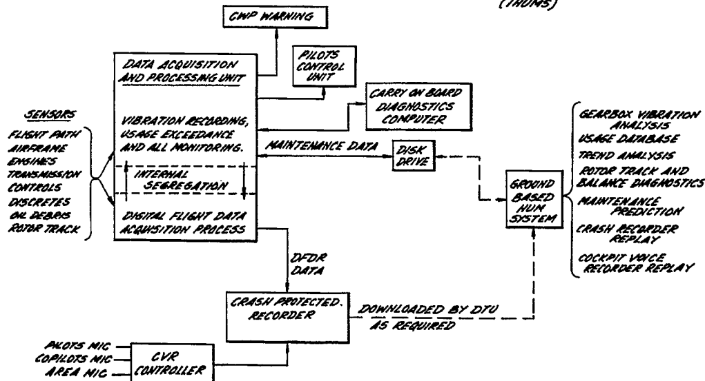
FIG. 1. BHL INTEGRATED FLIGHT RECORDING, HEALTH AND USAGE MONITORING SYSTEM (IHUINS)
