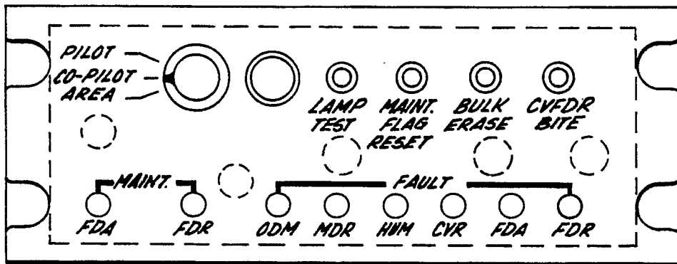
FIG. 12. THE I.M.P. PANEL
