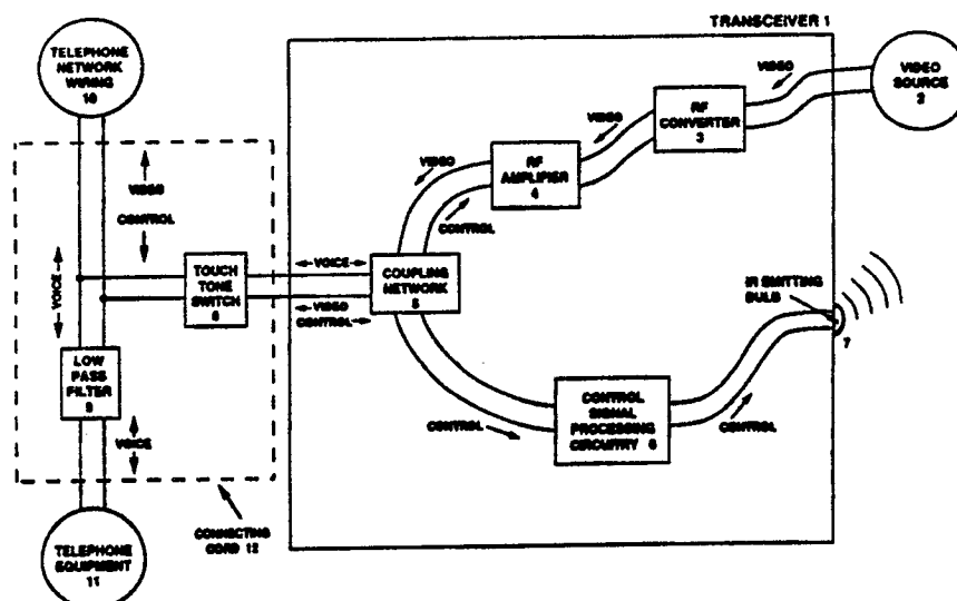
FIG.1 VIDEO SOURCE TRANSCIVER
