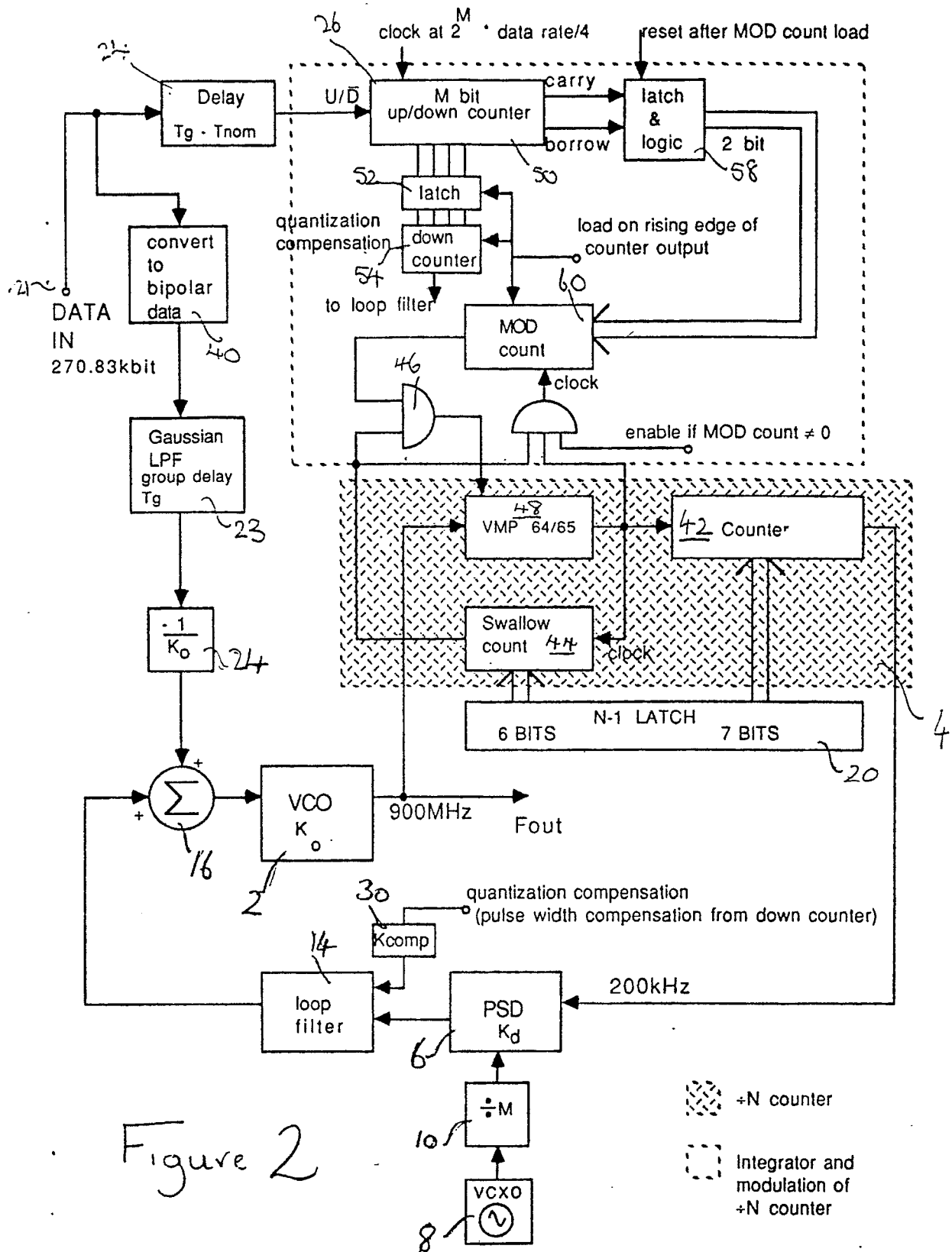
GMSK Modulated synthesiser (VCO & \div N modulation)
