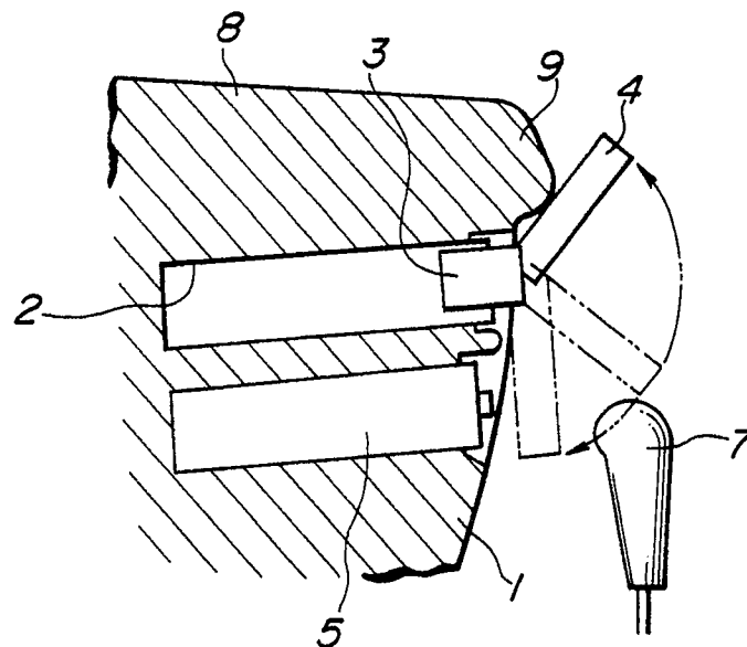
FIG. 12 (RELATED ART)
