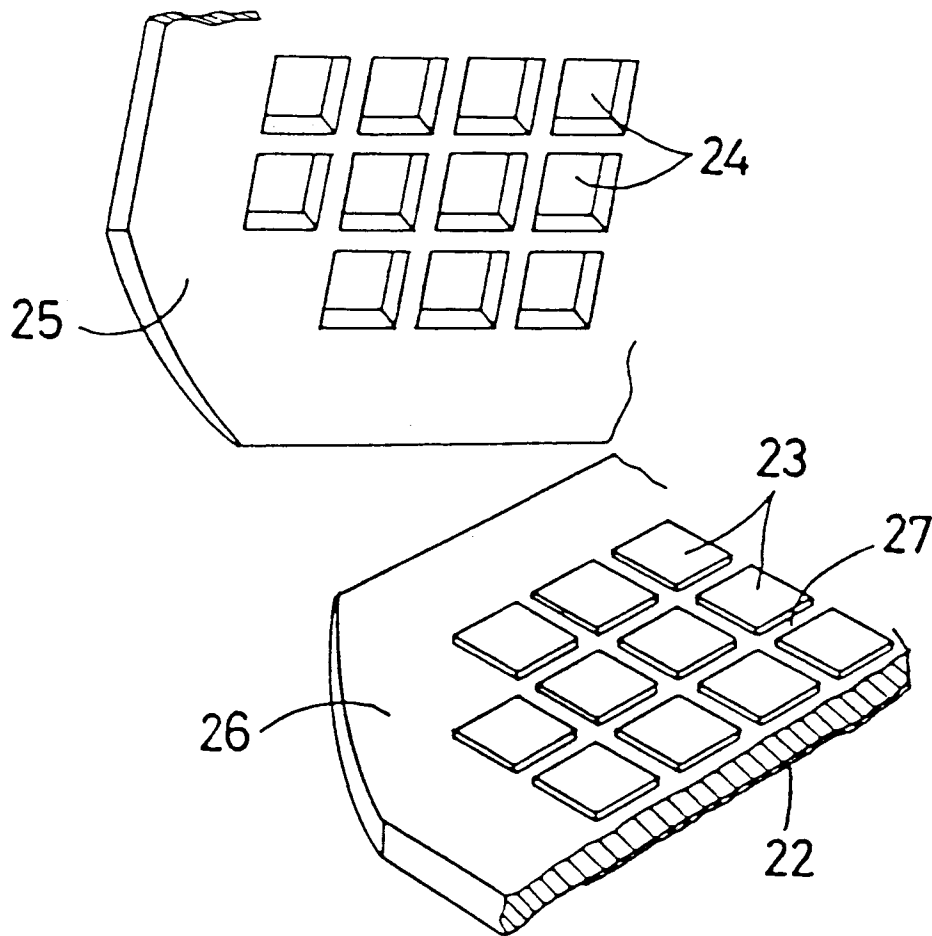
Fig.8 PRIOR ART
