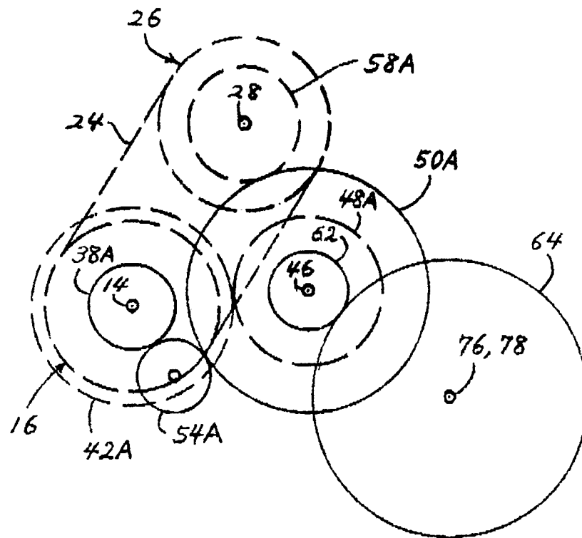
GEAR DRIVE (REVERSE)
