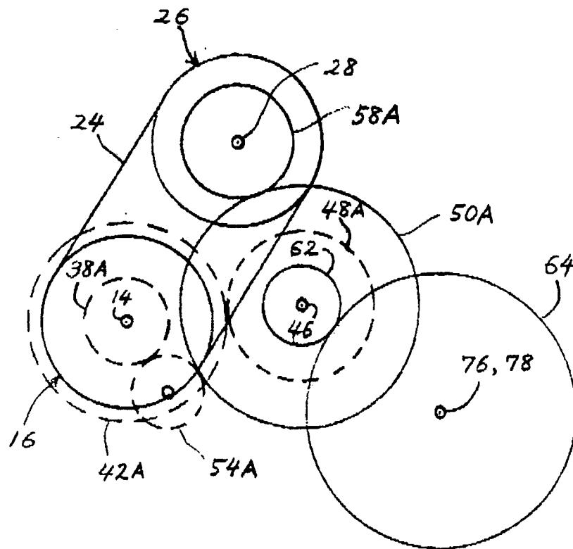
CVT DRIVE
