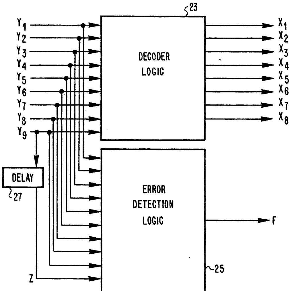
FIG. 6B (4,6,4) DECODER
