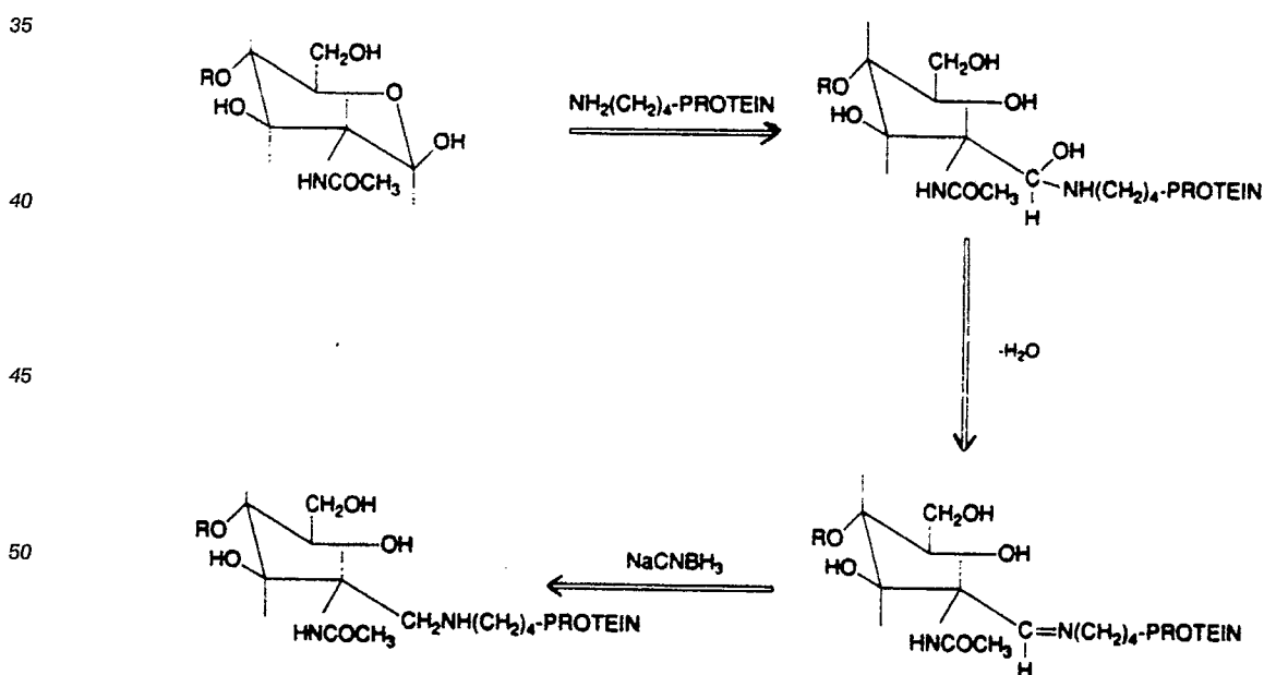
NEOGLYCOPROTEIN FORMATION BY REDUCTIVE AMINATION
