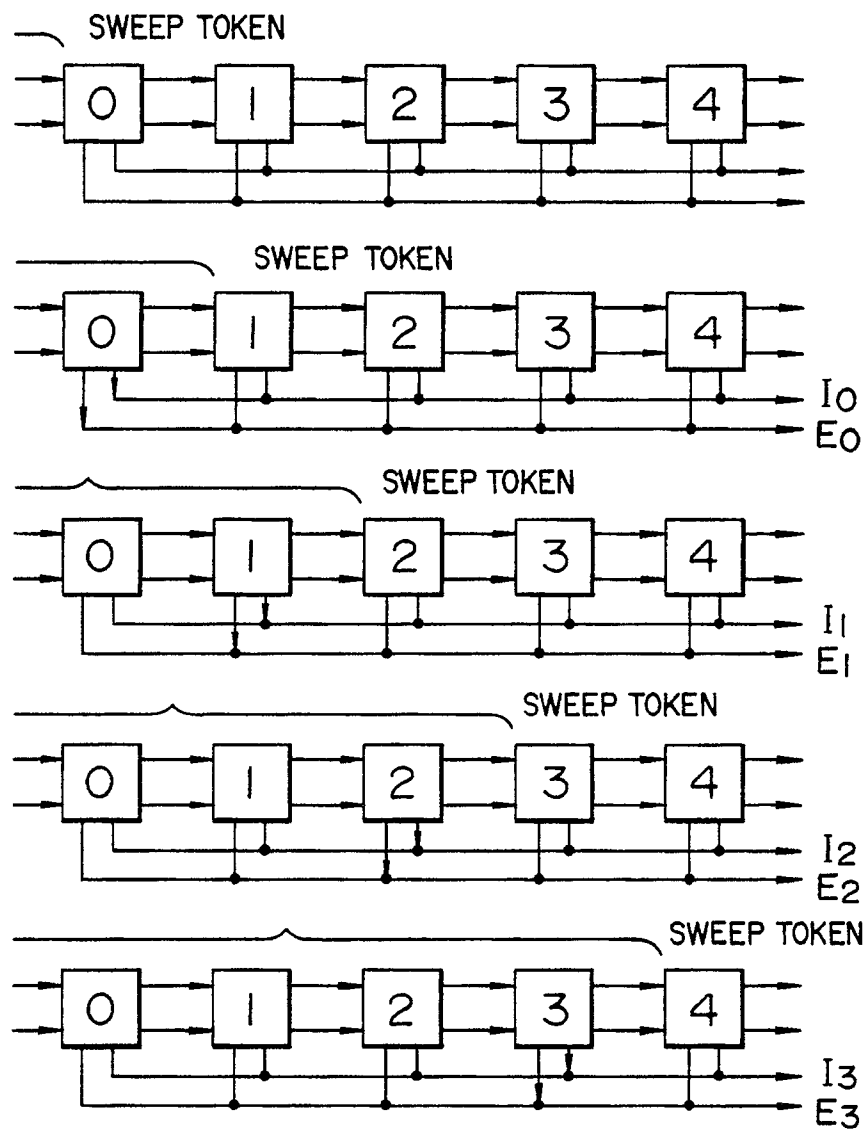
FIG. 4B FLOW OF SWEEP TOKEN
