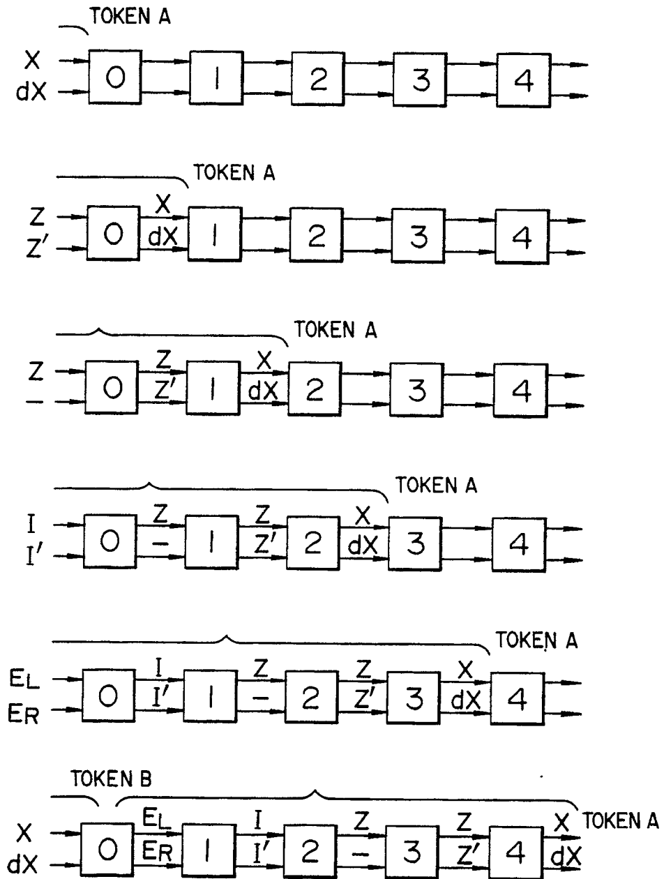
FIG. 4A FLOW OF SEGMENT TOKEN
