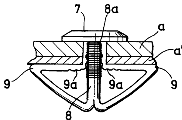
FIG.10(c) (PRIOR ART)
