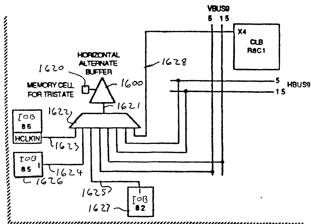
Inputs to the Horizontal Alternate Buffer
