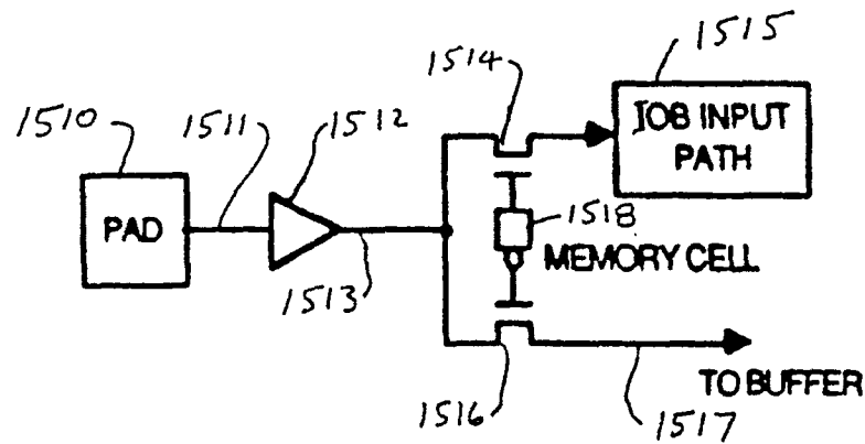
Special input to global buffers
