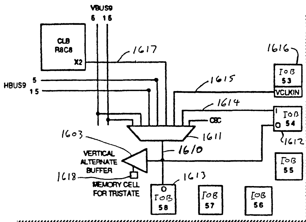
Inputs to the Vertical Alternate Buffer
