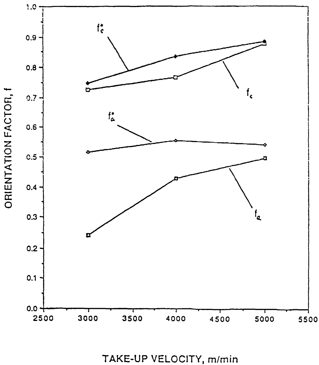
Fig. 9. Effect of OLZH on crystalline and amorphous orientation factors ( f , w/o OLZH, f^* , with OLZH).
