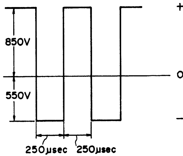
WAVEFORM OF SUPPLY 11
