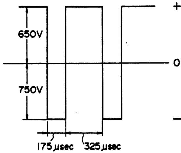
WAVEFORM OF SUPPLY 7
