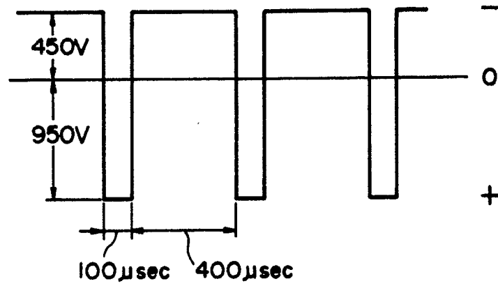
WAVEFORM OF SUPPLY 10
