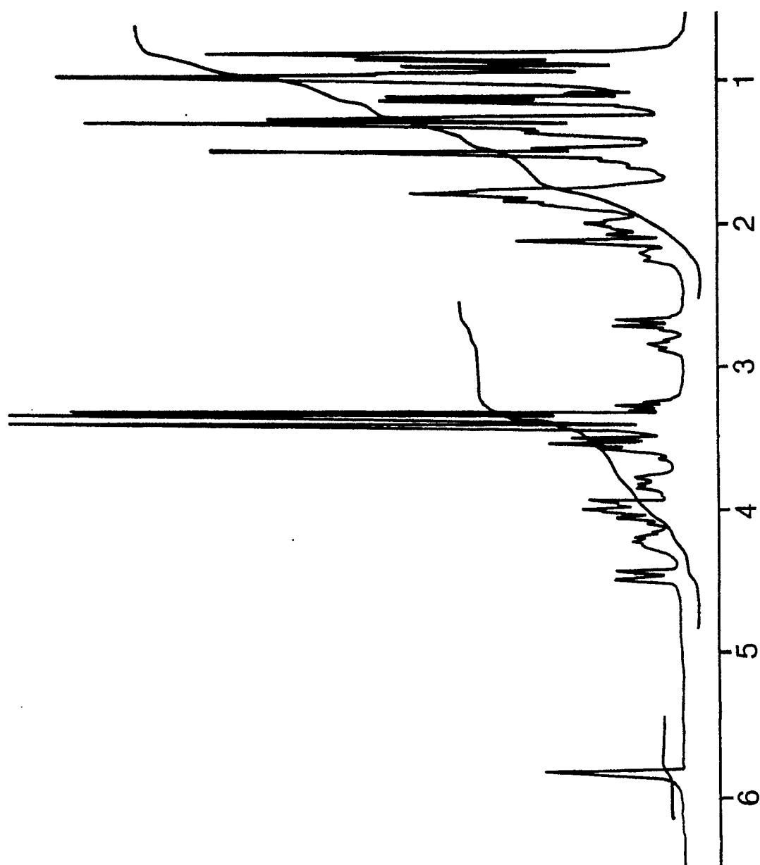
FIG.2. NMR Spectrum of A80789 (CDCl 3 )
