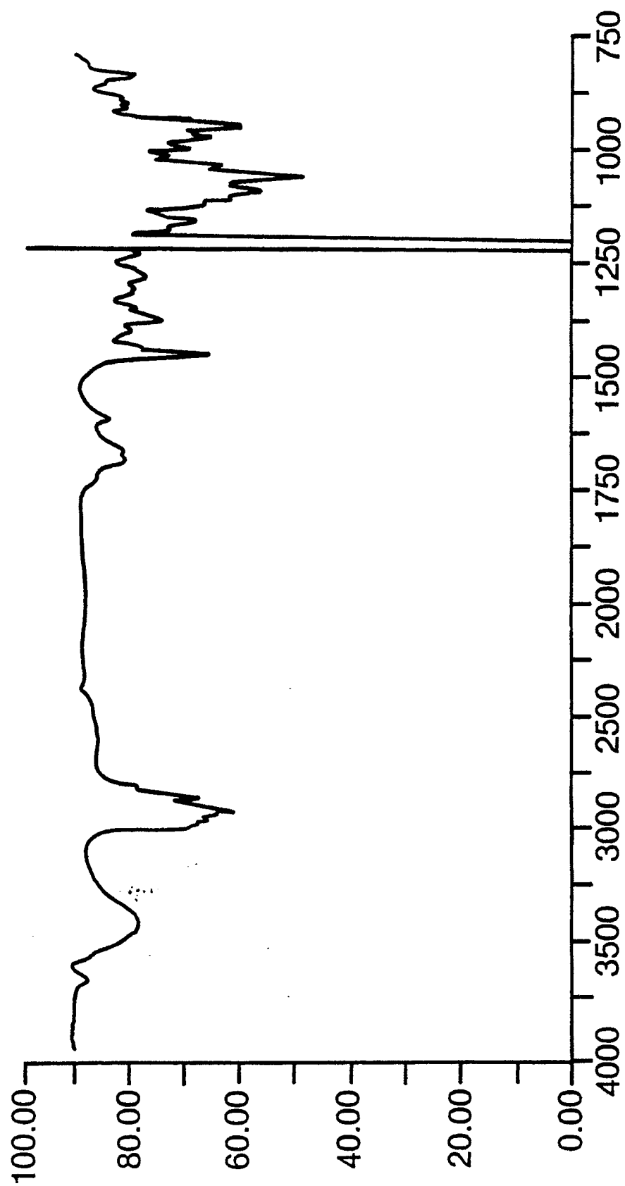
FIG.1. IR Spectrum of A80789 ( \text{CHCl}_3 )
