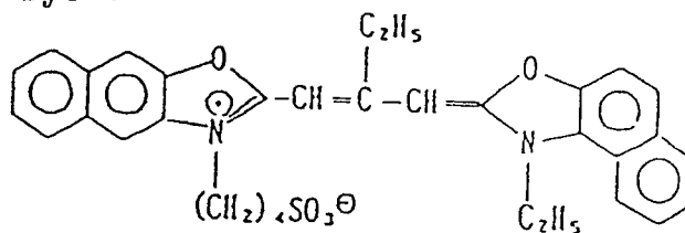
Sensitizing Dye VI
