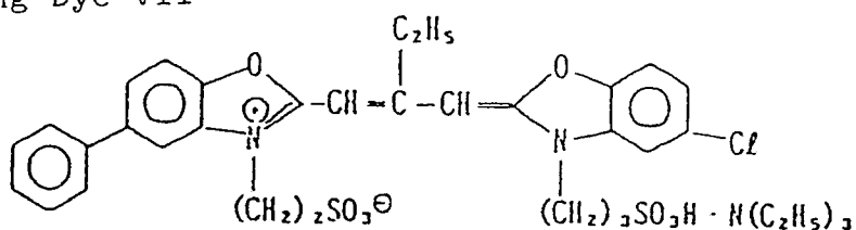
Sensitizing Dye VII
