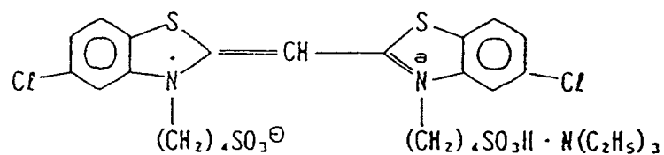
Sensitizing Dye VIII
