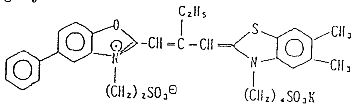
Sensitizing Dye V
