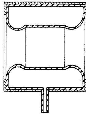
Fig. 18b ( PRIOR ART )
