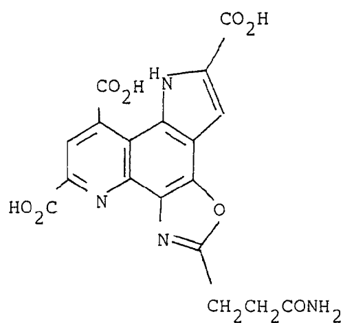
5-(2-Carbamoylethyl)-2,8,10-tricarboxy-1H-oxazo[5,4-h]-pyrrolo [ 2,3-f]quinoline. (8) 2-Methylthioethyl OPQ
