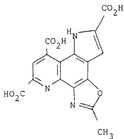
5-Methyl-2,8,10-tricarboxy-1H-oxazo[5,4-h]-pyrrolo[2,3-f]quinoline. (6) 2-Carboxylethyl OPQ
