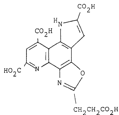
5-(2-Carboxylethyl)-2,8,10-tricarboxy-1H-oxazo[5,4-h]-pyrrolo[2,3-f]quinoline. (7) 2-Carbamoylethyl OPQ
