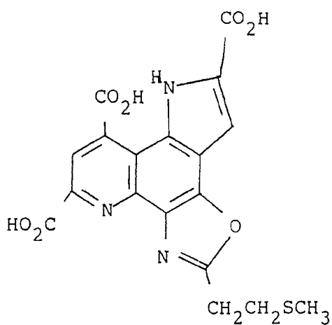
5-(2-Methylthioethyl)-2,8,10-tricarboxy-1H-oxazo[5,4-h]-pyrrolo [ 2,3-f]quinoline. (9) Benzyl OPQ
