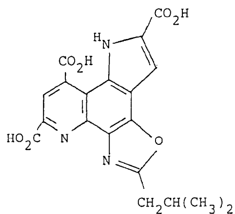
5-(2-Methylpropyl)-2,8,10-tricarboxy-1H-oxazo[5,4-h]-pyrrolo[2,3-f]quinoline. (5) Methyl OPQ
