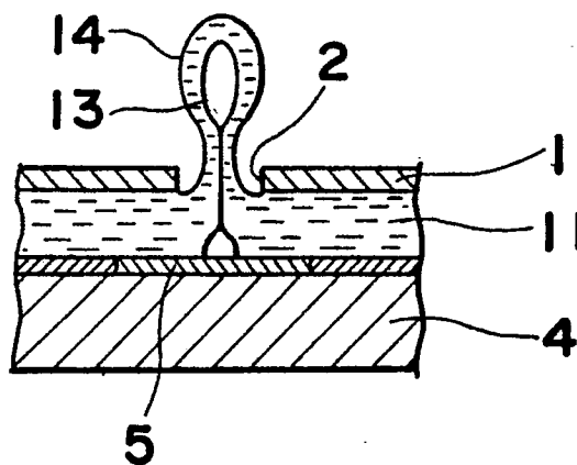
Fig. 15c PRIOR ART
