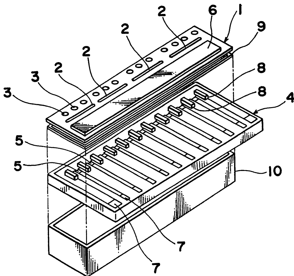
Fig. 14 PRIOR ART
