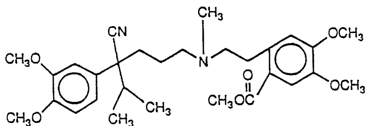
methyl 2-[2-[[4-cyano-4-(3,4-dimethoxyphenyl)-5-methylhexyl]methylamino]ethyl]-4,5-dimethoxybenzoate
