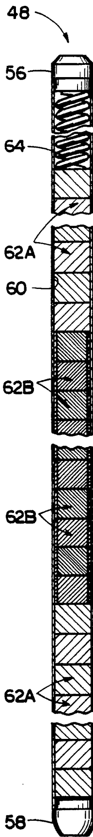
FIG. 4 (PRIOR ART)
