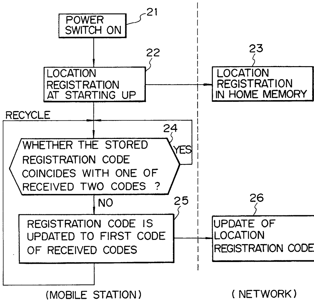
OPERATION FLOW-CHART IN THE FIRST EMBODIMENT
