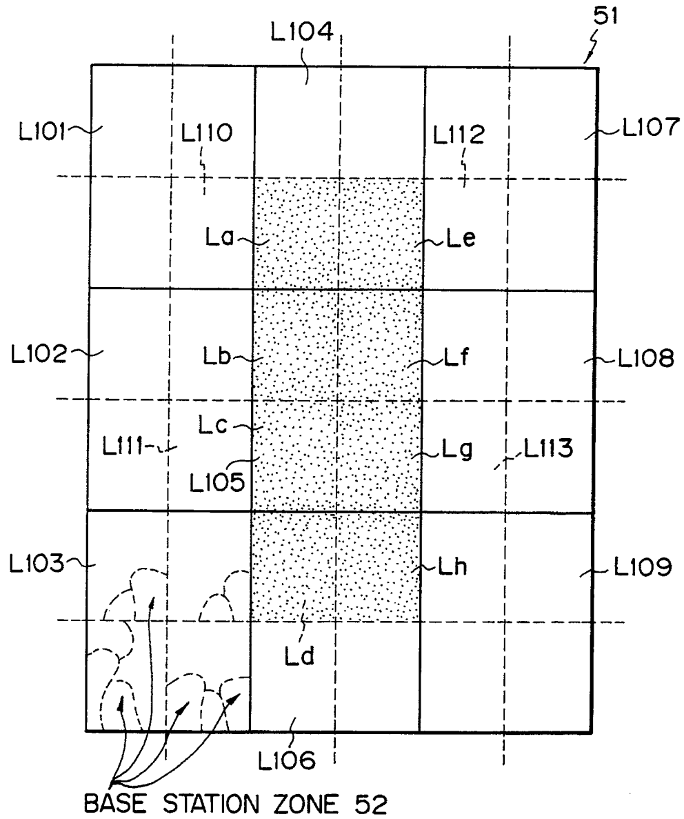
LOCATION REGISTRATION AREA IN SECOND EMBODIMENT
