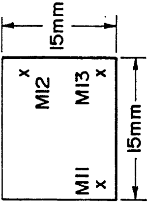
FIG. 11B MASK PATTERN
