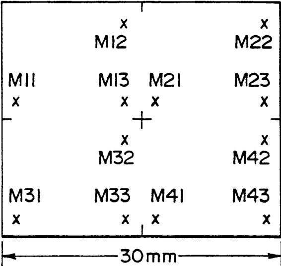
FIG. 15B MASK PATTERN
