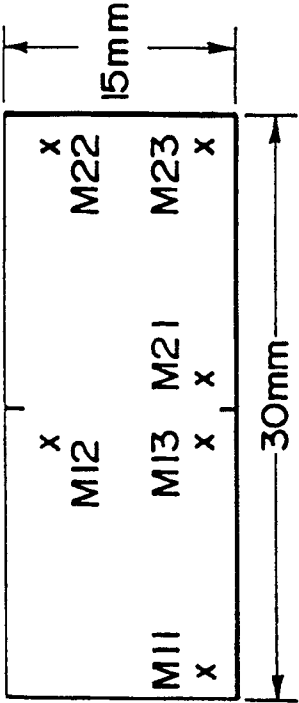
FIG. 10B MASK PATTERN
