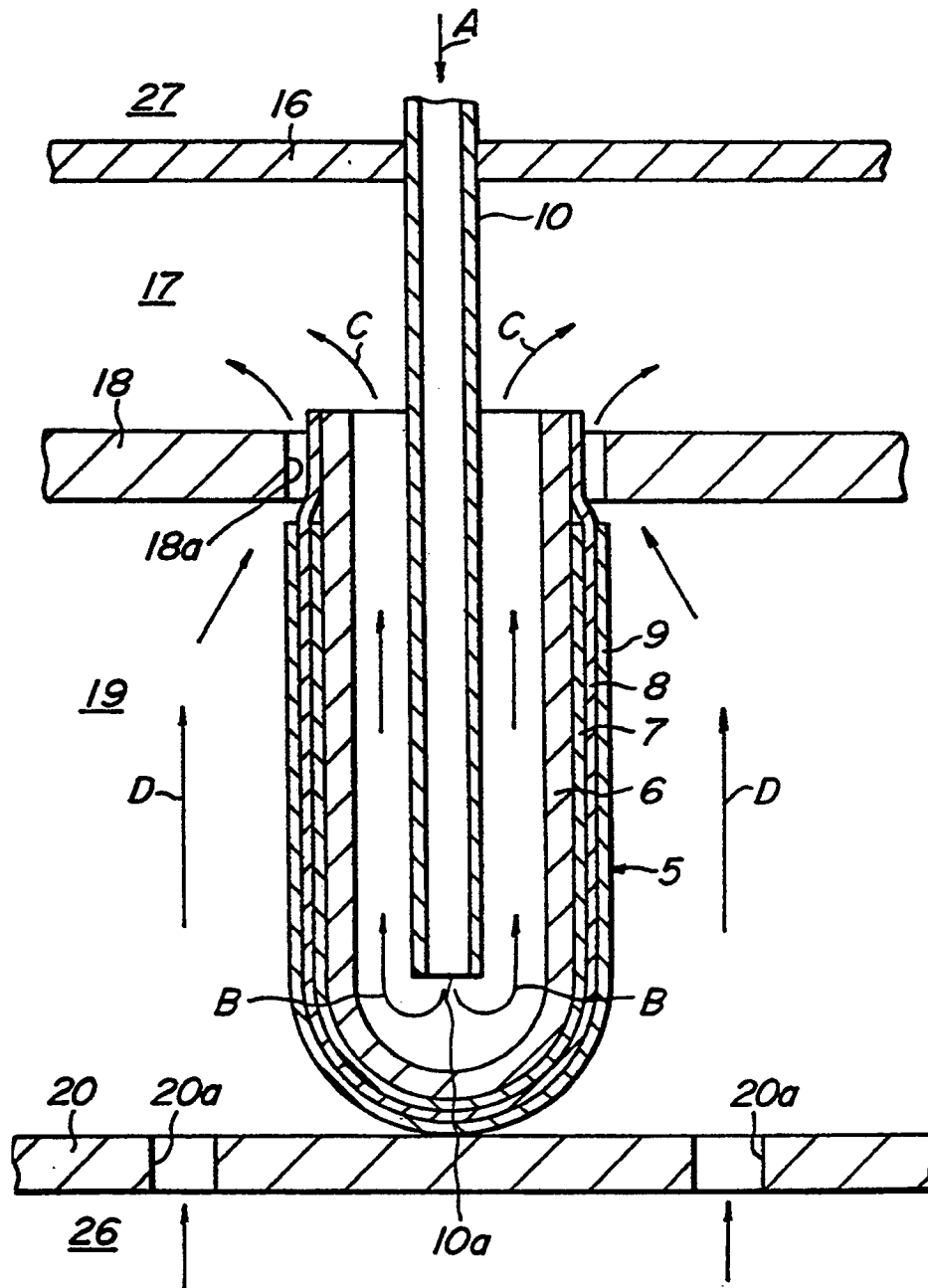
FIG. 6 PRIOR ART
