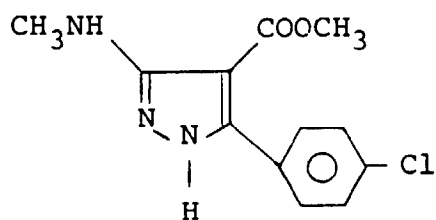
Compound C.
