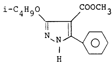
Compound D.
