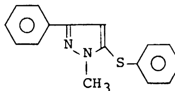
Compound B.
