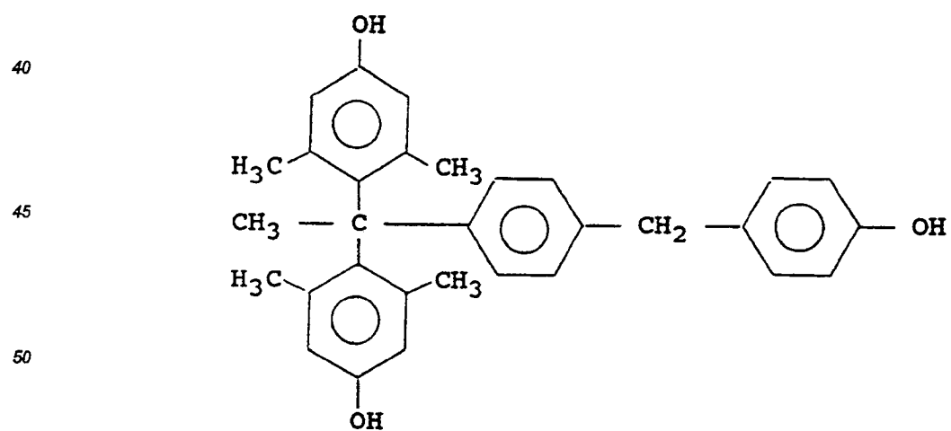
55 1,1-bis(3,4-dihydroxyphenyl)-1-[4-(4-hydroxybenzyl)phenyl]ethane
