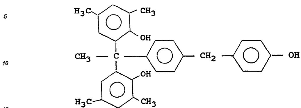
1,1-bis(4-hydroxy-3-methylphenyl)-1-[4-(4-hydroxybenzyl)phenyl]ethane
