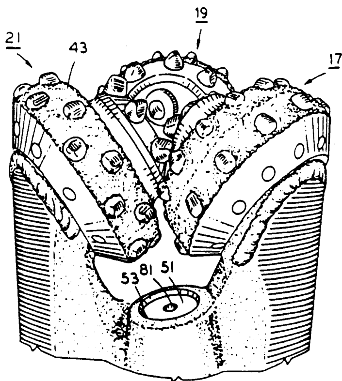
Fig. 2 PRIOR ART
