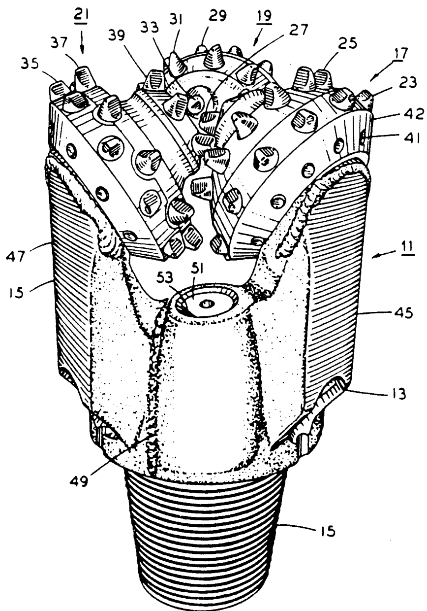
Fig. 1 PRIOR ART
