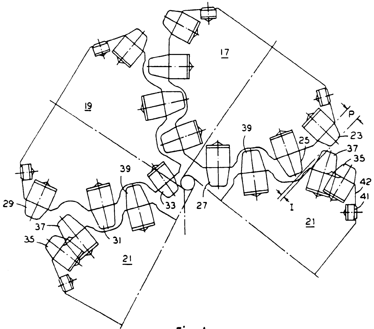
Fig. 4 PRIOR ART
