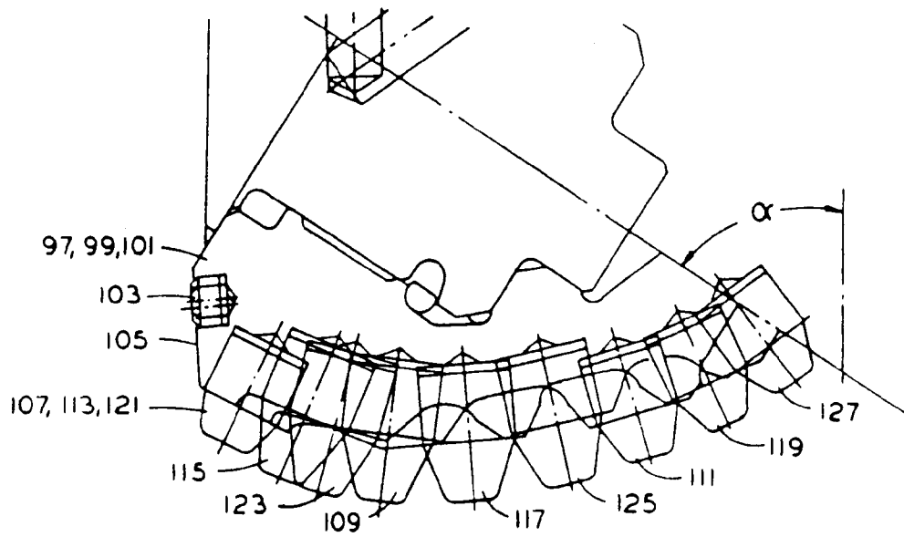
Fig. 6 PRIOR ART
