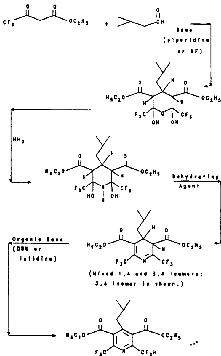
Scheme 1
