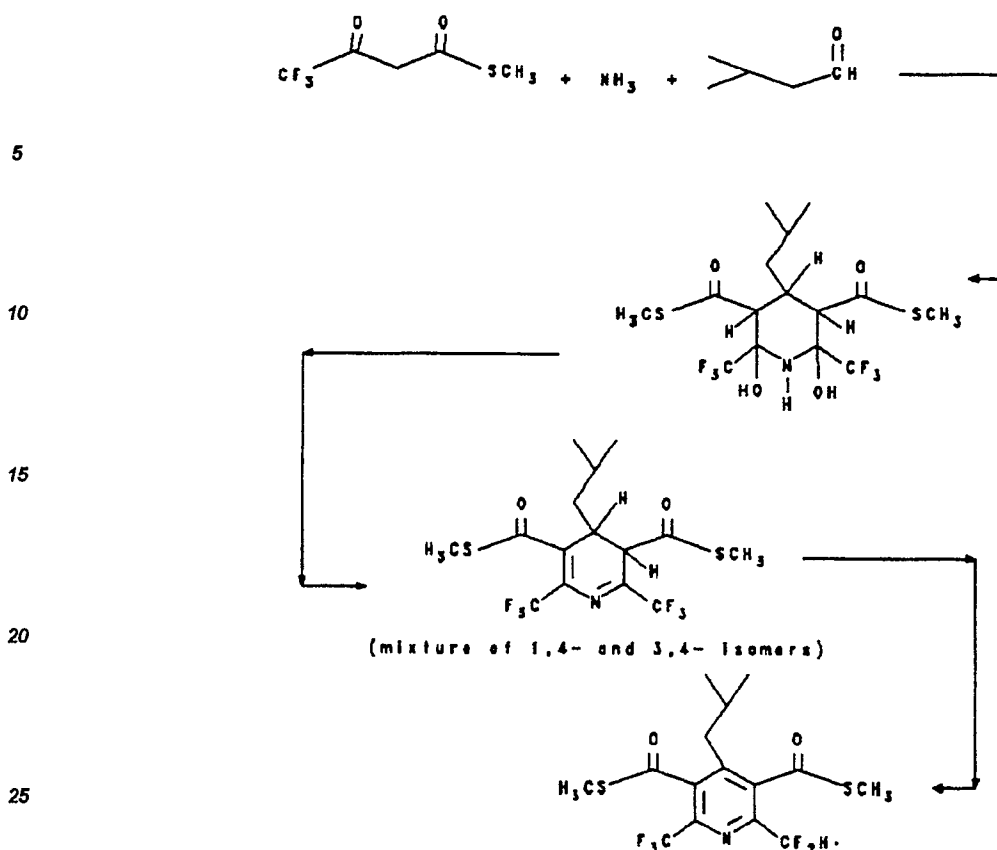
Scheme II
