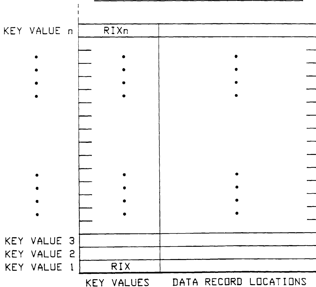
FIG. 12C INDEX FILE ORGANIZATION
