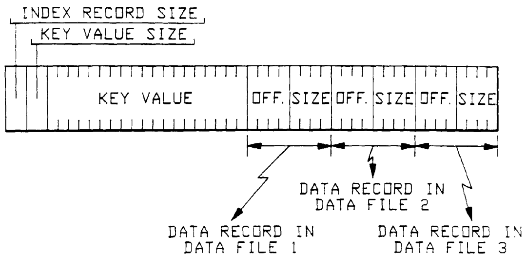
FIG. 12B INDEX RECORD STRUCTURE
