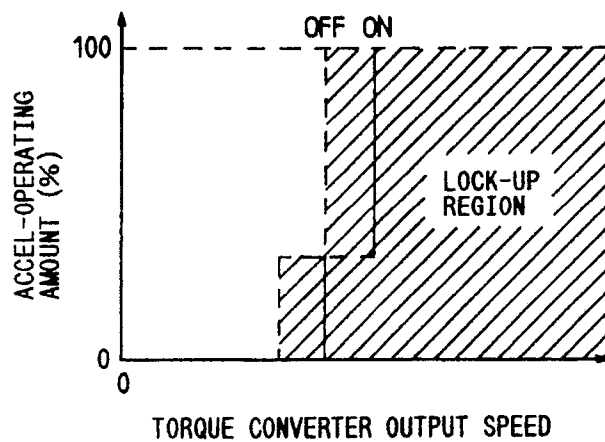
FIG. 50 PRIOR ART
