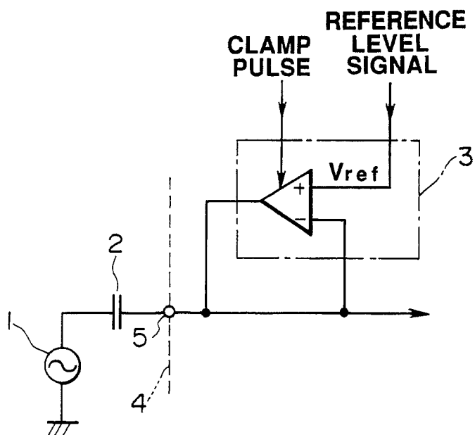
FIG. 5 (RELATED ART)
