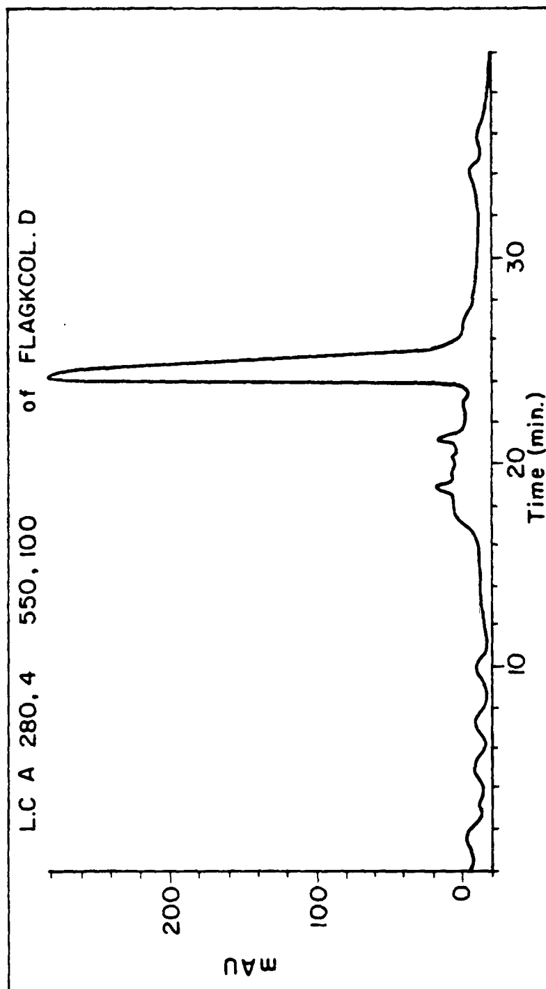
FIG. 8. A representative HPLC of purified pCBI2-10-6 showing a single major peak
