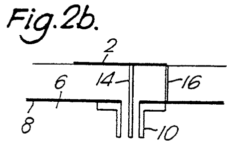
(b) SHORT-CIRCUITED QUARTER-WAVE RESONANT PATCH.
