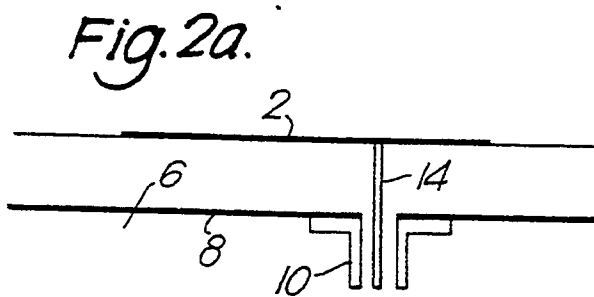
(a) HALF-WAVE RESONANT PATCH.
