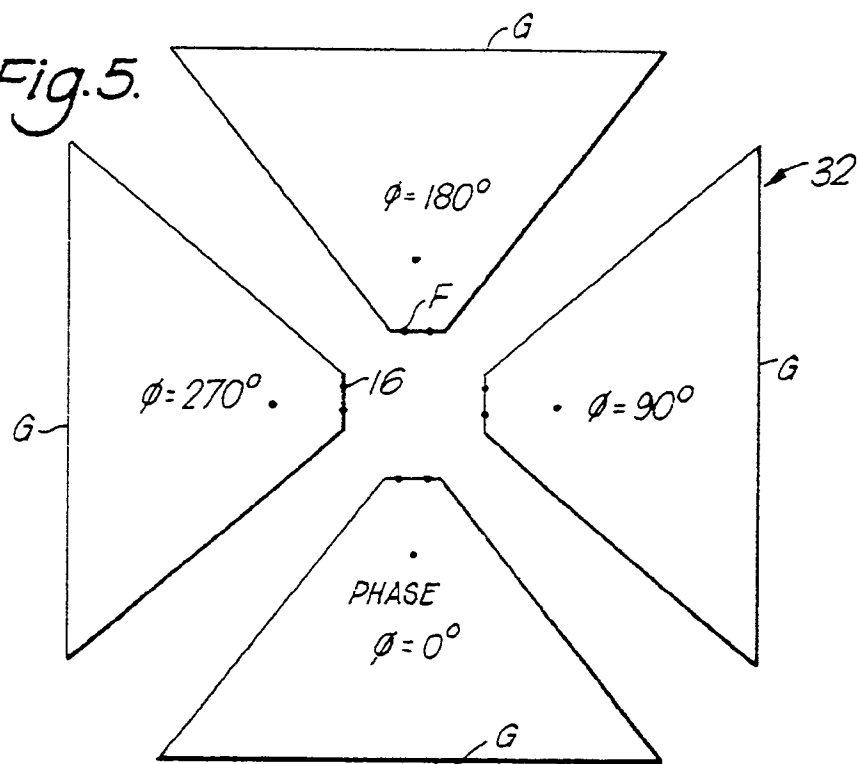
CIRCULARLY POLARISED FOUR-ELEMENT TRAPEZIUM ARRAY.
