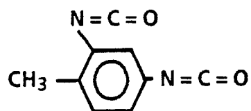
tolylene 2,4-diisocyanate ,
