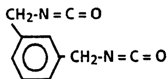
m-xylylene diisocyanate ,
