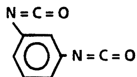
1,3-phenylene diisocyanate
