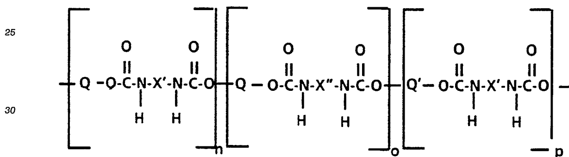
FORMULA I
