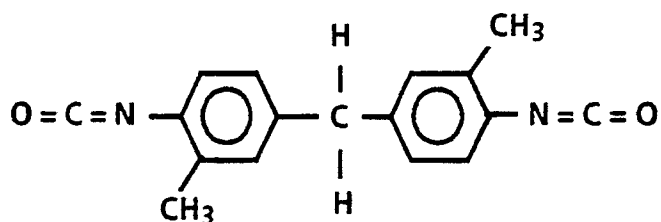
3,3'-dimethyldiphenylmethane-4,4'-diisocyanate)
