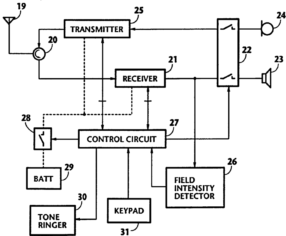
FIG. 4 CORDLESS STATION 5
