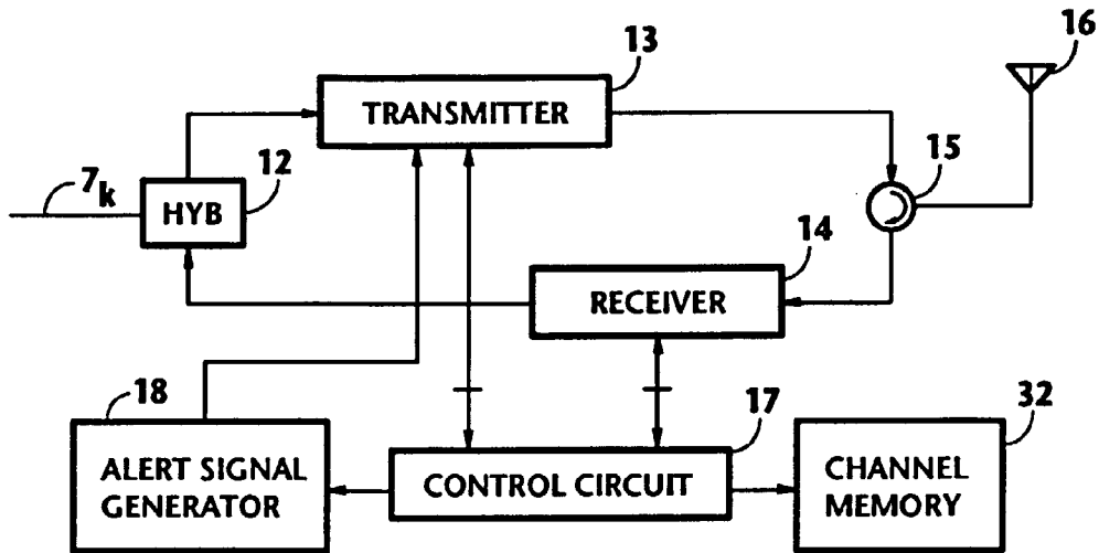
FIG. 3 ACCESS UNIT 4 k
