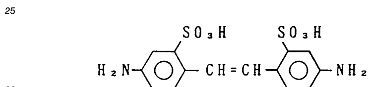
diaminobenzylsulfonic acid
