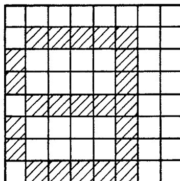
REPLACEMENT DATA
