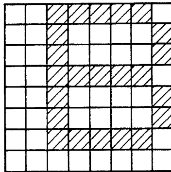
NORMAL DATA
