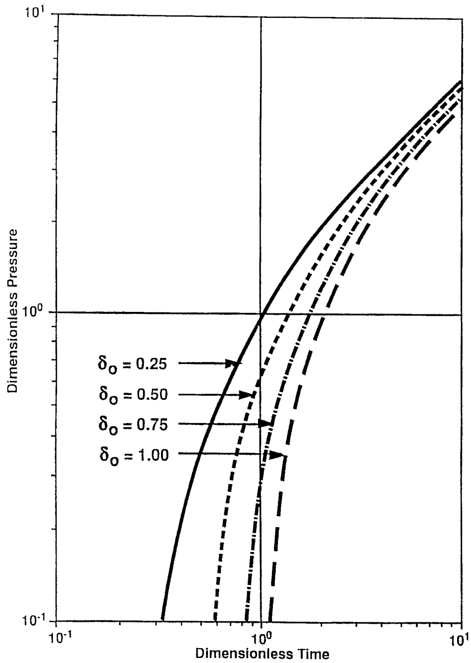
Fig. 1-Type Curve for Leakoff Exponent = 0.50
