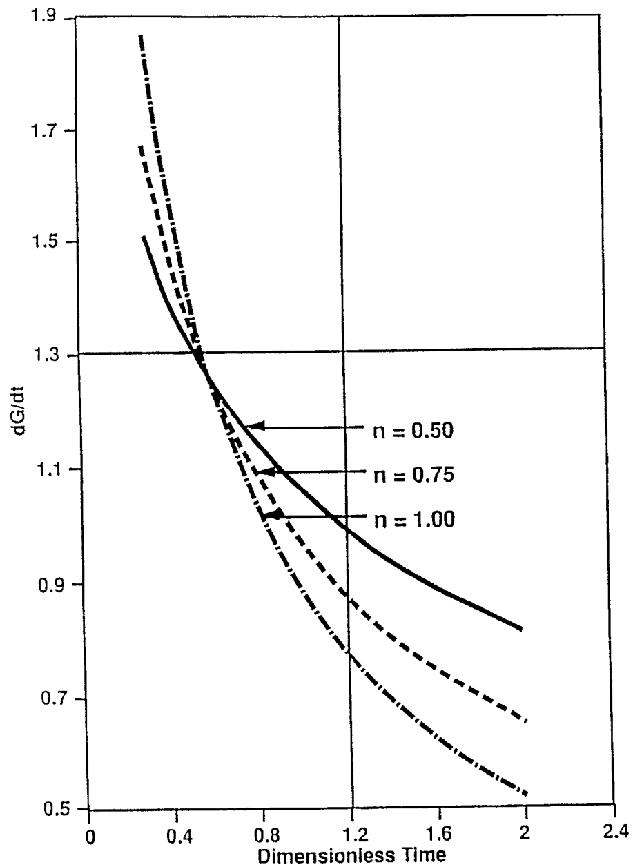
Fig. 6-Derivative of Dimensionless Pressure
