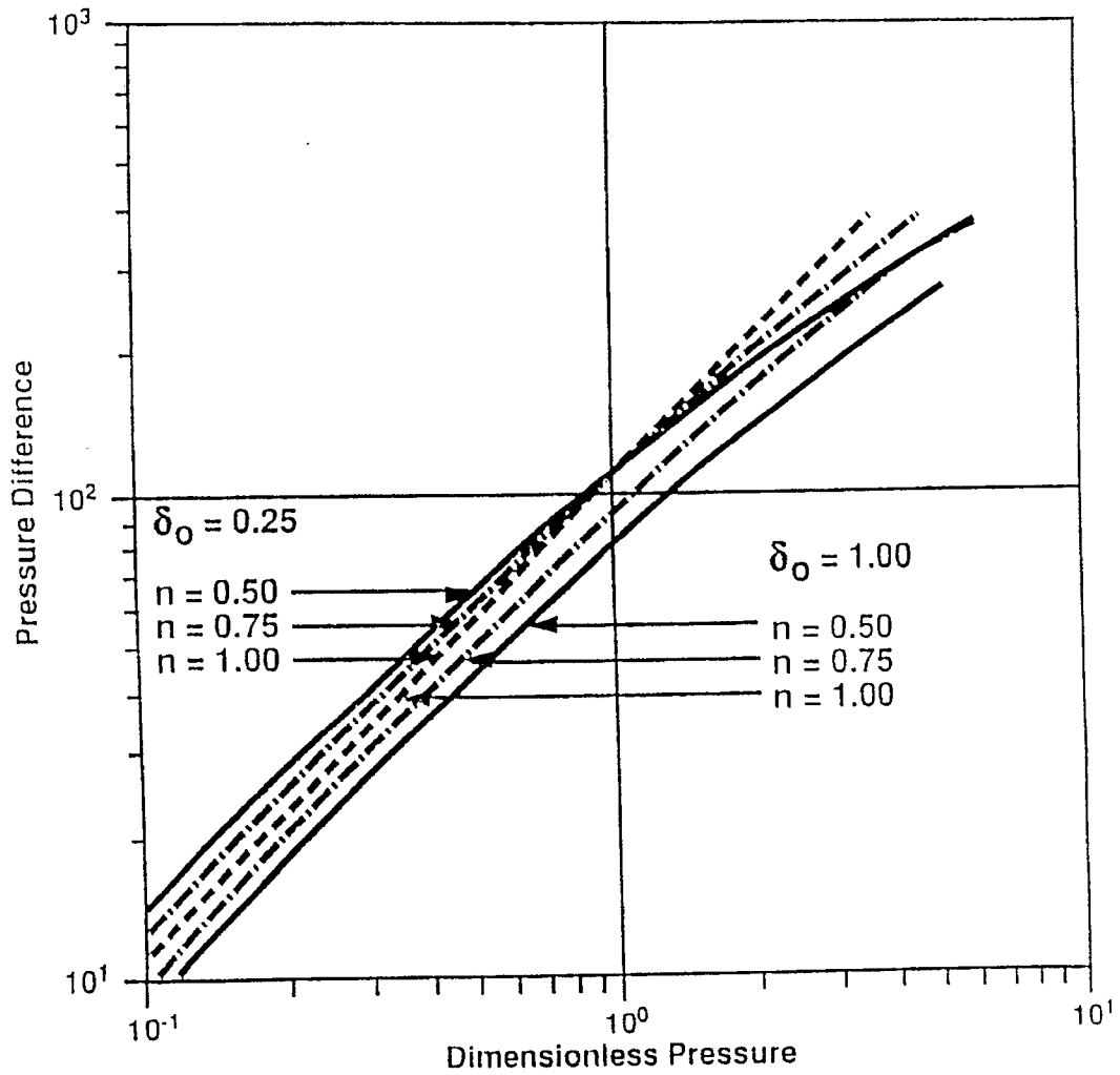
Fig. 5 - Pressure Difference vs Dimensionless Pressure
