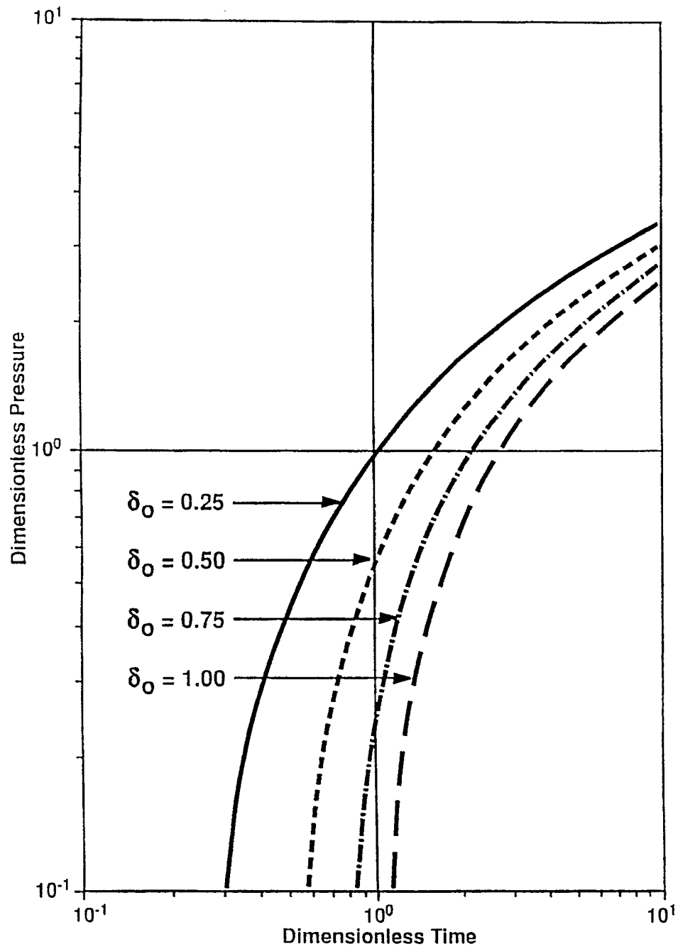
Fig. 3-Type Curve for Leak-off Exponent = 1.00
