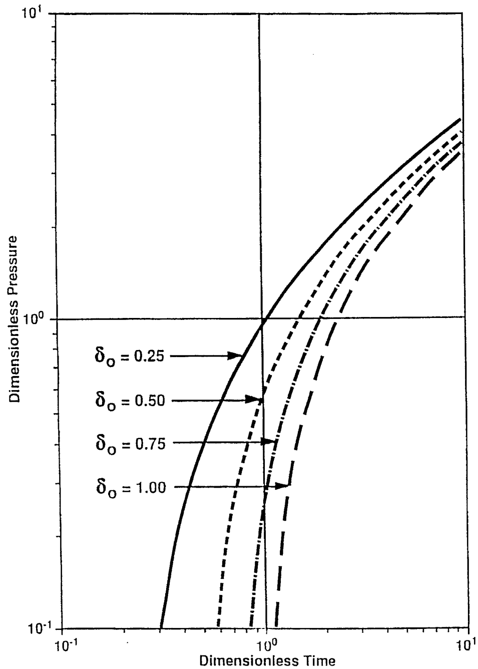
Fig. 2-Type Curve for Leak-off Exponent = 0.75
