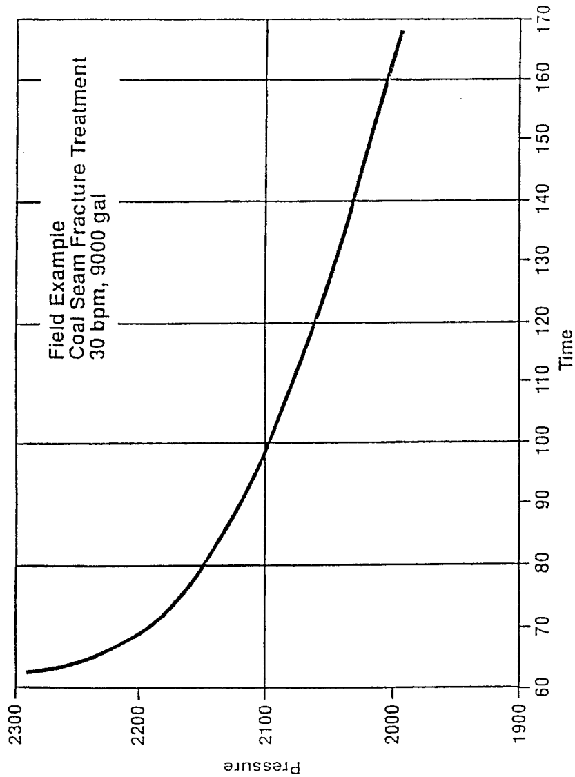
Fig. 7-Pressure Decline vs Time
