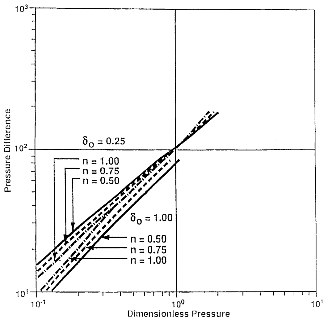
Fig. 9 -Pressure Difference vs Dimensionless Pressure
