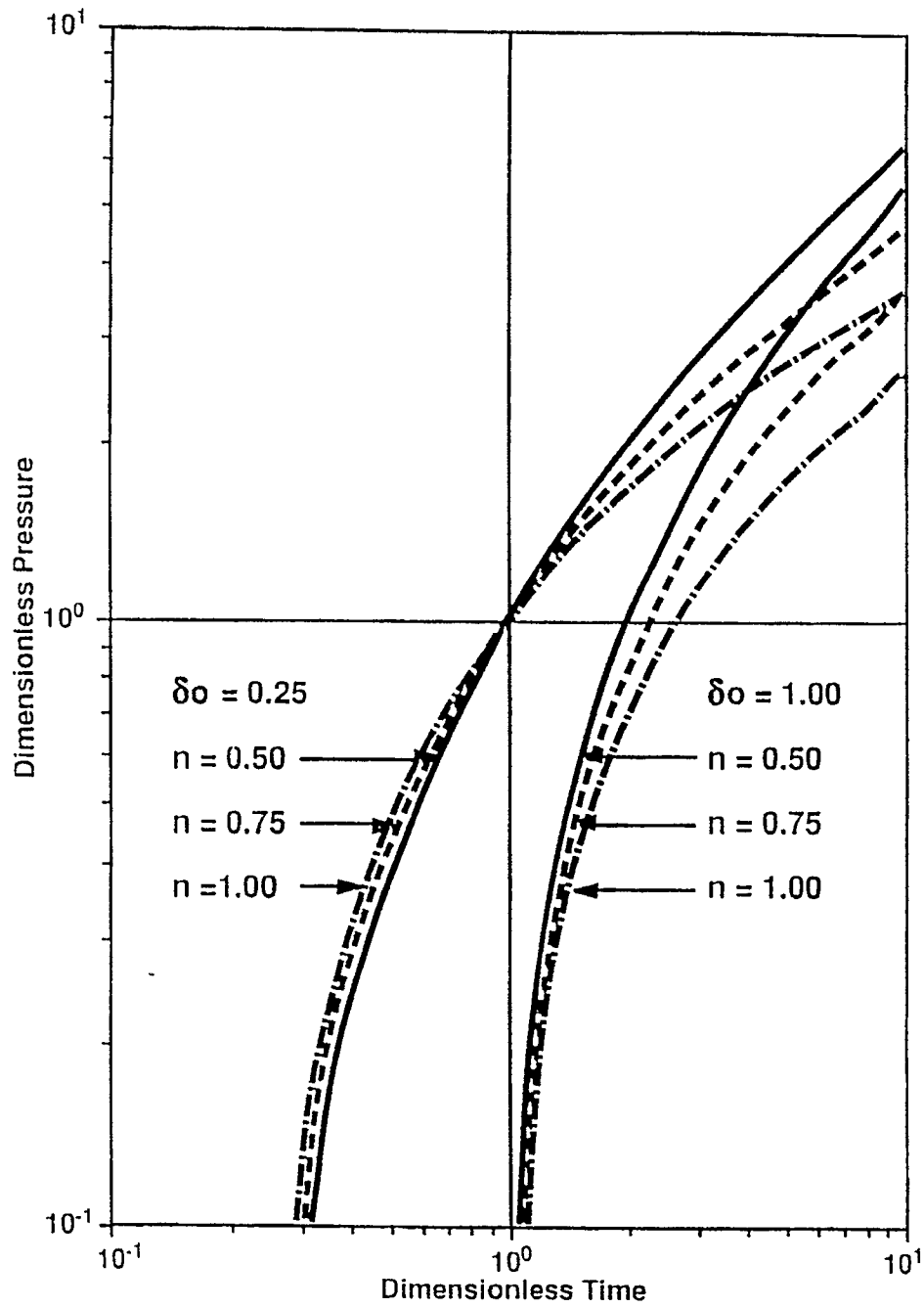
Fig. 4-Comparison of Type Curves
