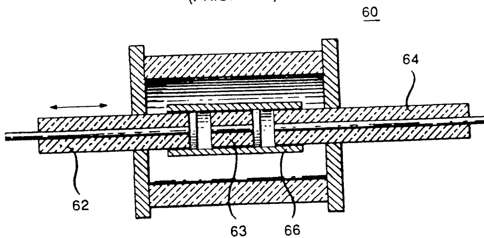
FIG. 6 (PRIOR ART)
